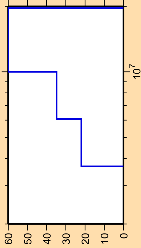
\Delta\sigma/\sigma vs. E for ^{169}\text{Dy}(n,n\text{cont.})
