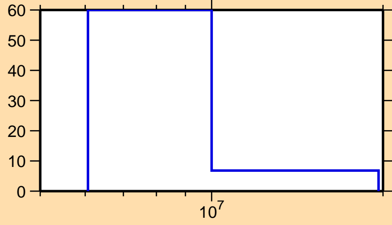
\Delta\sigma/\sigma vs. E for ^{169}\text{Dy}(n,el.)
