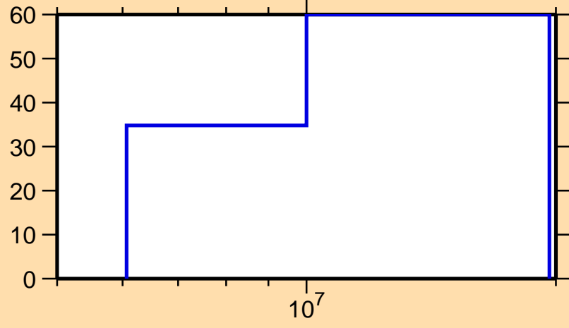
\Delta\sigma/\sigma vs. E for ^{169}\text{Dy}(n,ncont.)
