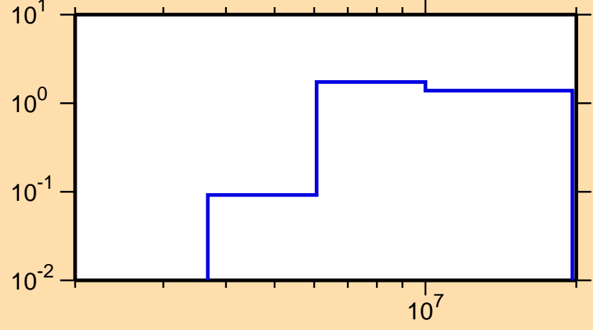
\sigma vs. E for ^{169}\text{Dy}(n,2n)
