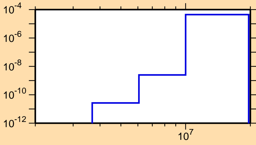
\sigma vs. E for ^{169}\text{Dy}(n,\alpha)
