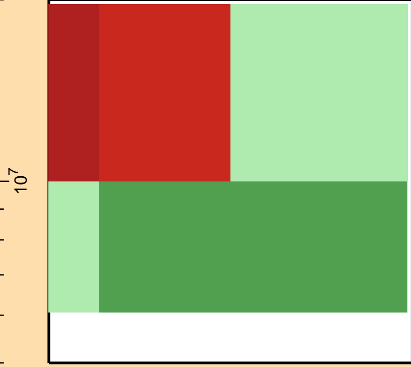
\Delta\sigma/\sigma vs. E for ^{169}\text{Dy}(n,\gamma)
