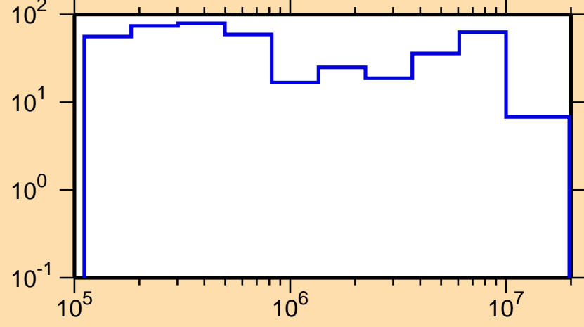
\Delta\sigma/\sigma vs. E for ^{169}\text{Dy}(n,\text{el.})
