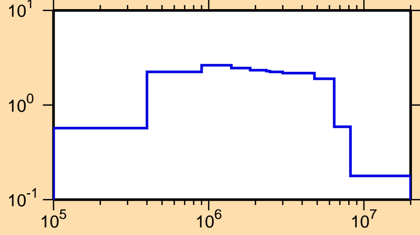
\sigma vs. E for ^{169}\text{Dy}(n,\text{inel.})
