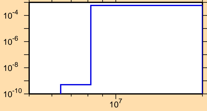
\sigma vs. E for ^{169}\text{Dy}(n,p)
