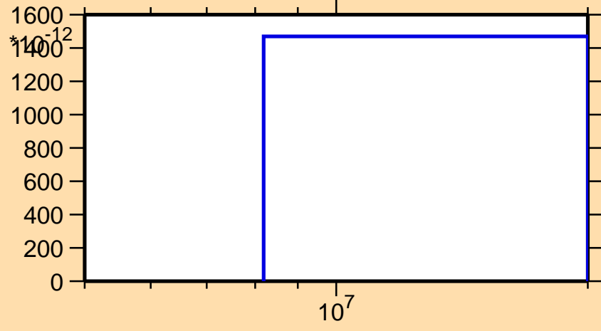
\sigma vs. E for ^{169}\text{Dy}(n,\text{nd})
