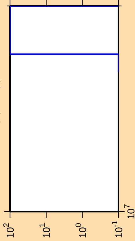
\Delta\sigma/\sigma vs. E for ^{170}\text{Dy}(n,2np)
