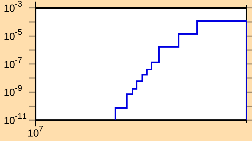
\sigma vs. E for ^{170}\text{Dy}(n,np)
