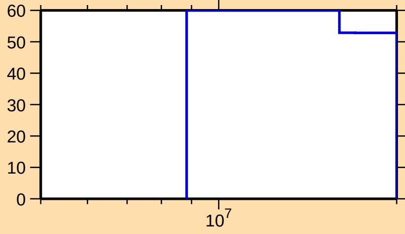
\Delta\sigma/\sigma vs. E for ^{170}\text{Dy}(n,n_1)
