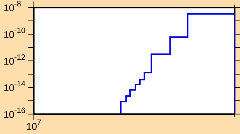
\sigma vs. E for ^{170}\text{Dy}(n,2n\alpha)
