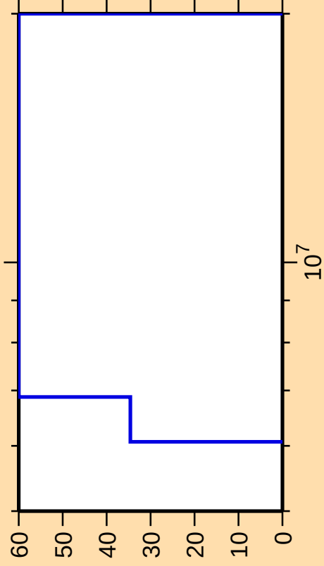
\Delta\sigma/\sigma vs. E for ^{170}\text{Dy}(n,n\text{cont.})
