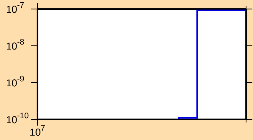
\sigma vs. E for ^{170}\text{Dy}(n,nt)
