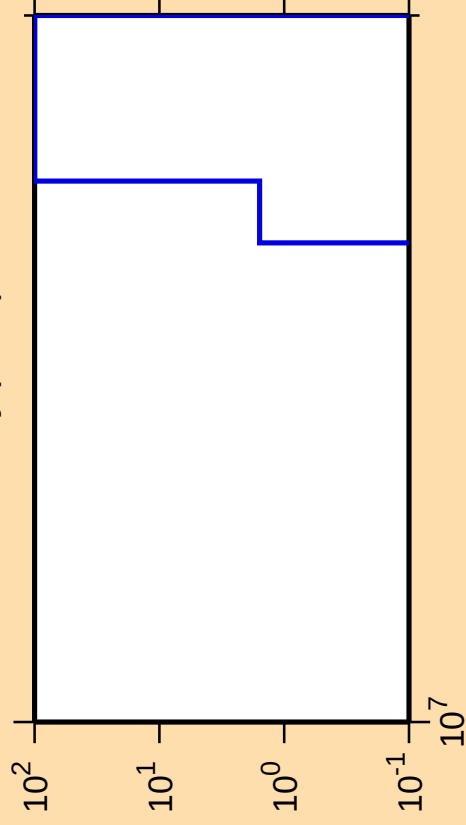
\Delta\sigma/\sigma vs. E for ^{170}\text{Dy}(n,\text{nd})
