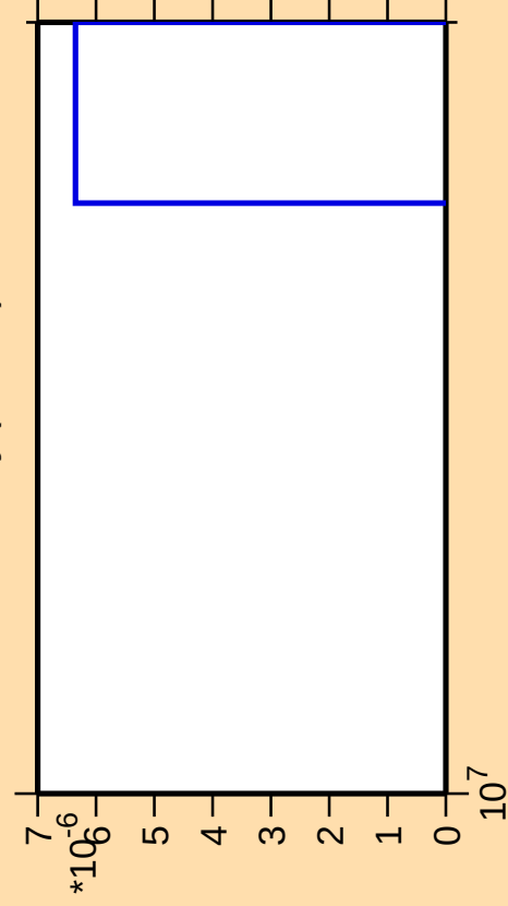
\Delta\sigma/\sigma vs. E for ^{170}\text{Dy} (mt 11)
