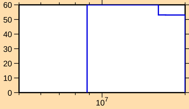
\Delta\sigma/\sigma vs. E for ^{170}\text{Dy}(n,\text{inel.})
