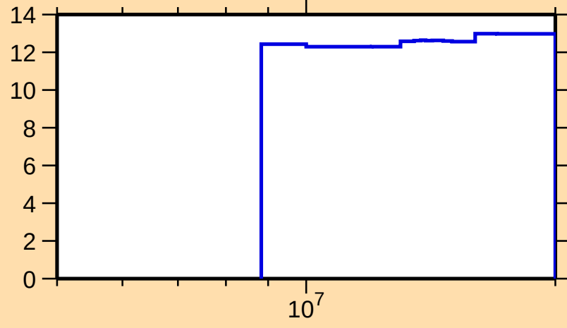
\Delta\sigma/\sigma vs. E for ^{170}\text{Dy}(n,\text{nonel.})
