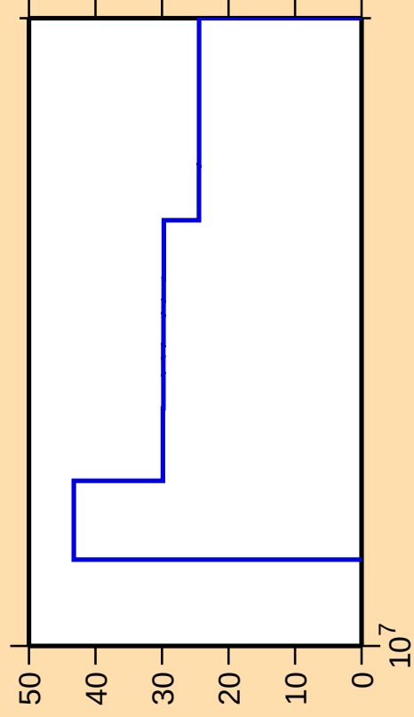
\Delta\sigma/\sigma vs. E for ^{170}\text{Dy}(n,3n)
