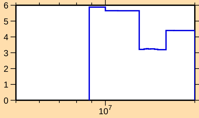
\Delta\sigma/\sigma vs. E for ^{170}\text{Dy}(n,\text{tot.})
