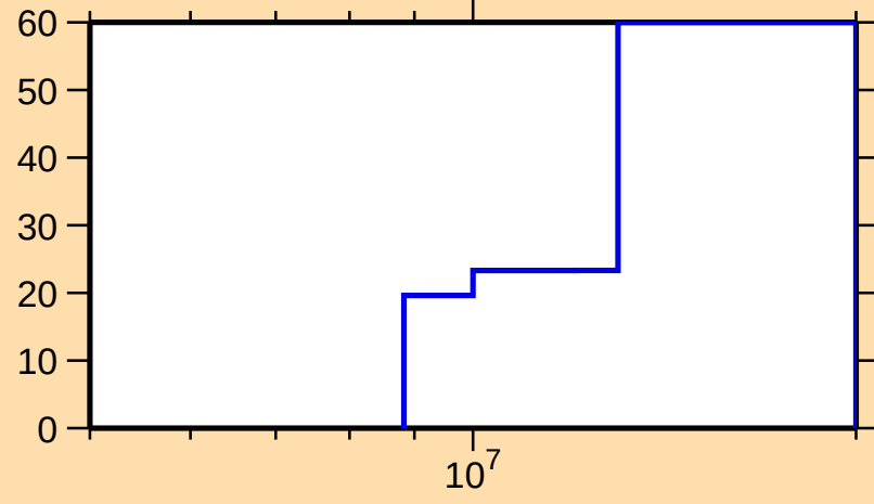
\Delta\sigma/\sigma vs. E for ^{170}\text{Dy}(n,2n)
