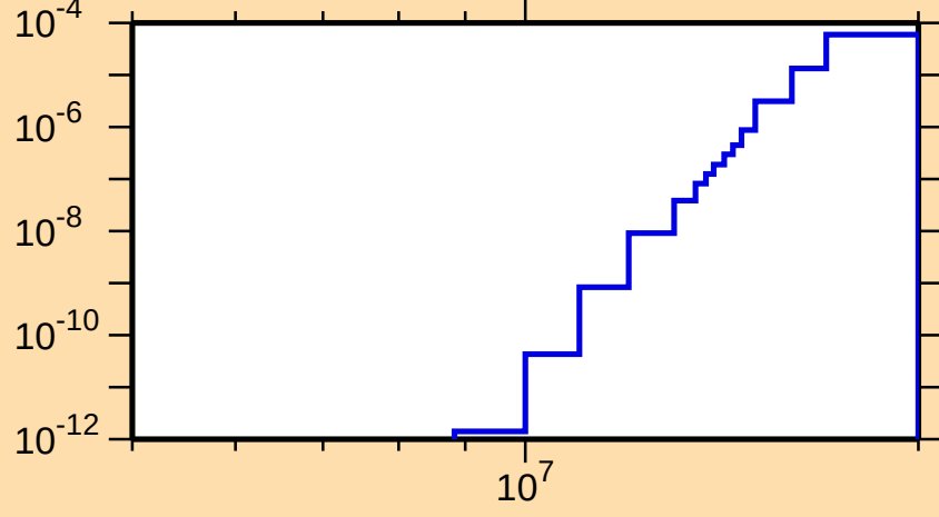
\sigma vs. E for ^{170}\text{Dy}(n,n\alpha)
