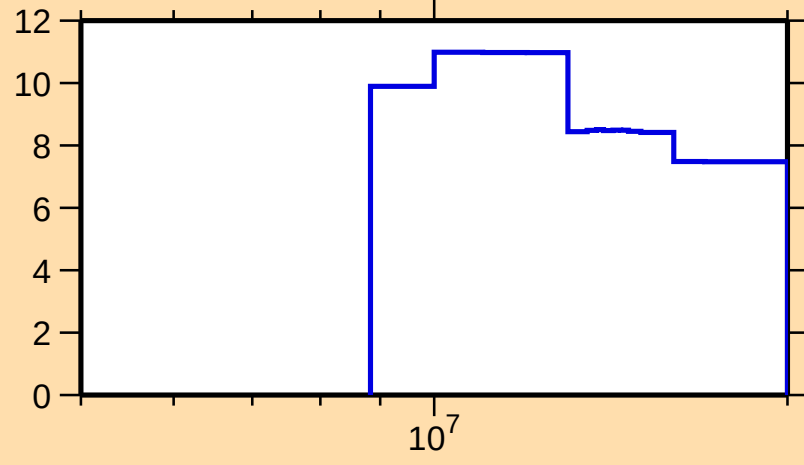
\Delta\sigma/\sigma vs. E for ^{170}\text{Dy}(n,\text{el.})
