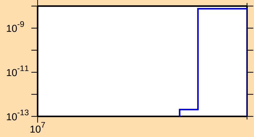
\sigma vs. E for ^{170}\text{Dy}(n,\text{nd})
