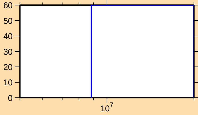
\Delta\sigma/\sigma vs. E for ^{170}\text{Dy}(n,n\text{cont.})
