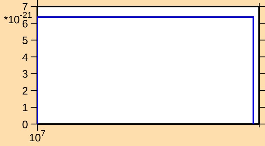
\sigma vs. E for ^{170}\text{Dy} (mt 11)
