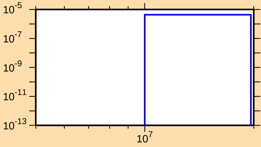
\sigma vs. E for ^{170}\text{Dy}(n,d)
