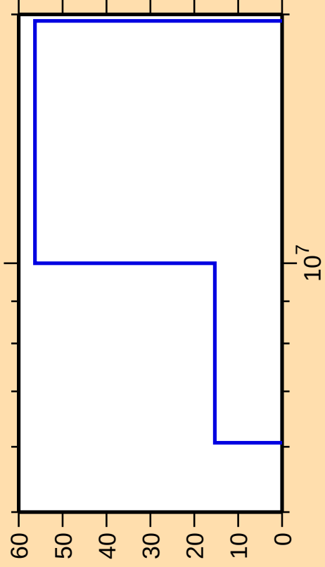
\Delta\sigma/\sigma vs. E for ^{170}\text{Dy}(n,2n)
