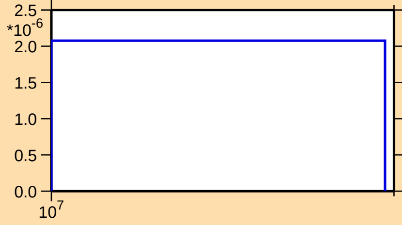
\sigma vs. E for ^{170}\text{Dy}(n,np)
