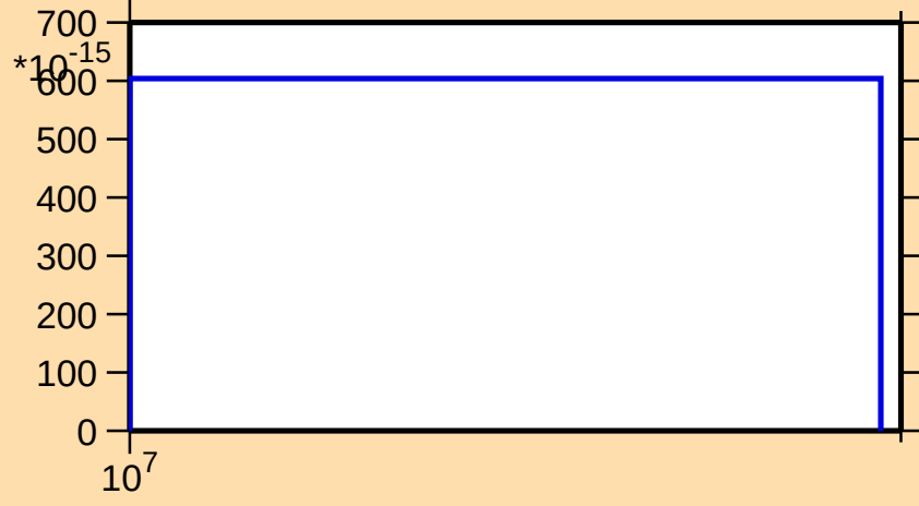
\sigma vs. E for ^{170}\text{Dy}(n,2np)
