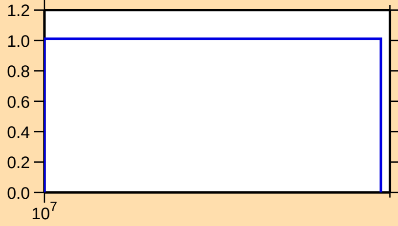
\sigma vs. E for ^{170}\text{Dy}(n,3n)
