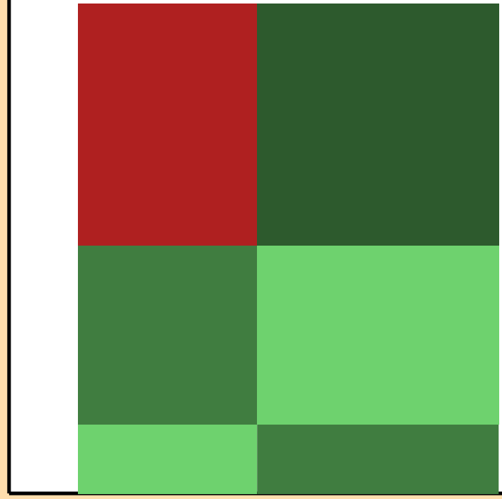
\Delta\sigma/\sigma vs. E for ^{170}\text{Dy}(n,2n)
