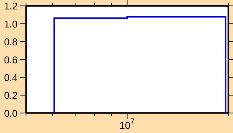
\sigma vs. E for ^{170}\text{Dy}(n,2n)
