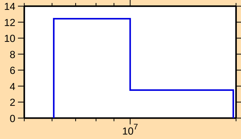
\Delta\sigma/\sigma vs. E for ^{170}\text{Dy}(n,\text{tot.})
