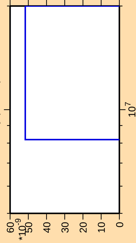
\Delta\sigma/\sigma vs. E for ^{170}\text{Dy}(\text{mt } 11)
