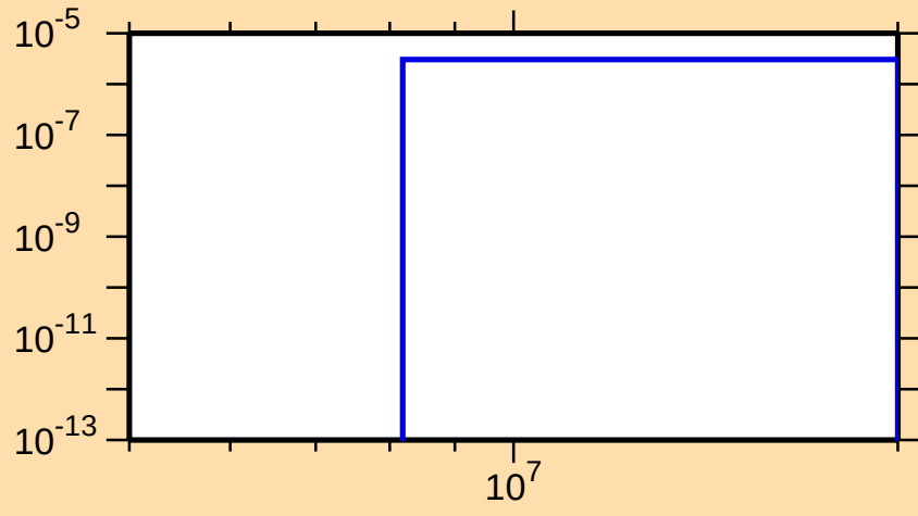
\sigma vs. E for ^{170}\text{Dy}(n,t)
