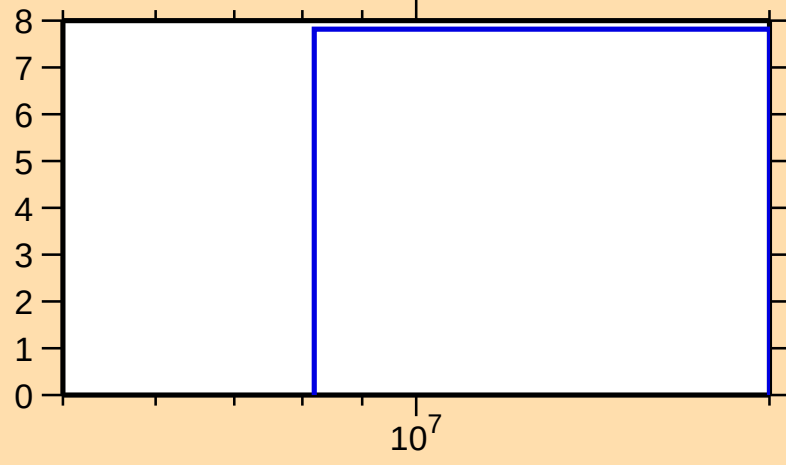
\Delta\sigma/\sigma vs. E for ^{170}\text{Dy}(n,\text{el.})
