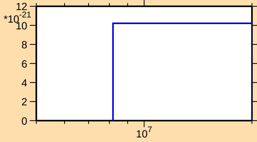
\sigma vs. E for ^{170}\text{Dy}(\text{mt } 11)
