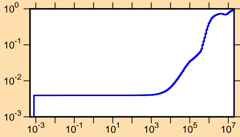
\mu vs. E for ^{171}\text{Dy}(\text{mt251})
