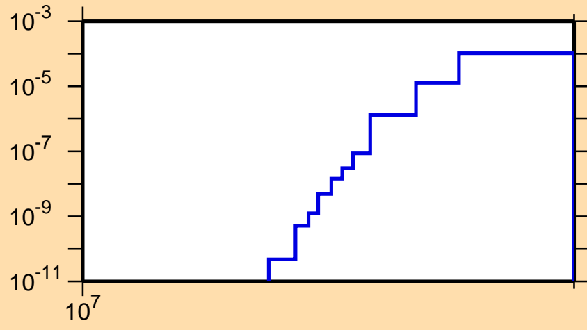
\sigma vs. E for ^{171}\text{Dy}(n,np)
