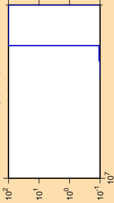
\Delta\sigma/\sigma vs. E for ^{171}\text{Dy}(n,2np)
