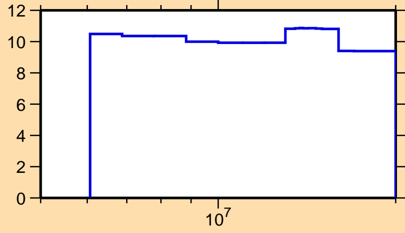
\Delta\sigma/\sigma vs. E for ^{171}\text{Dy}(n,\text{nonel.})
