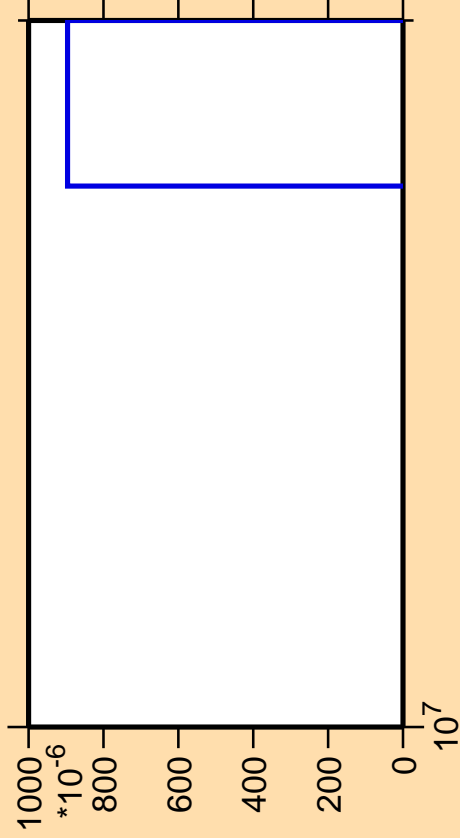
\Delta\sigma/\sigma vs. E for ^{171}\text{Dy} (mt 11)
