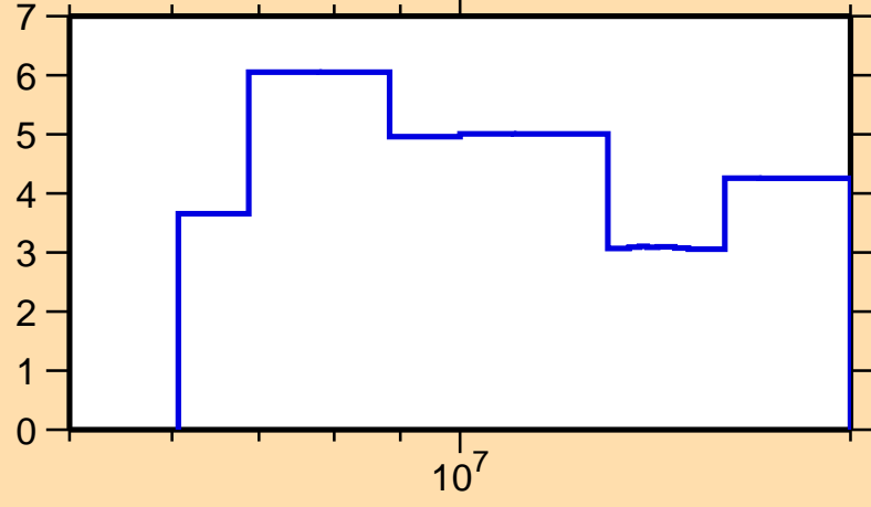
\Delta\sigma/\sigma vs. E for ^{171}\text{Dy}(n,\text{tot.})
