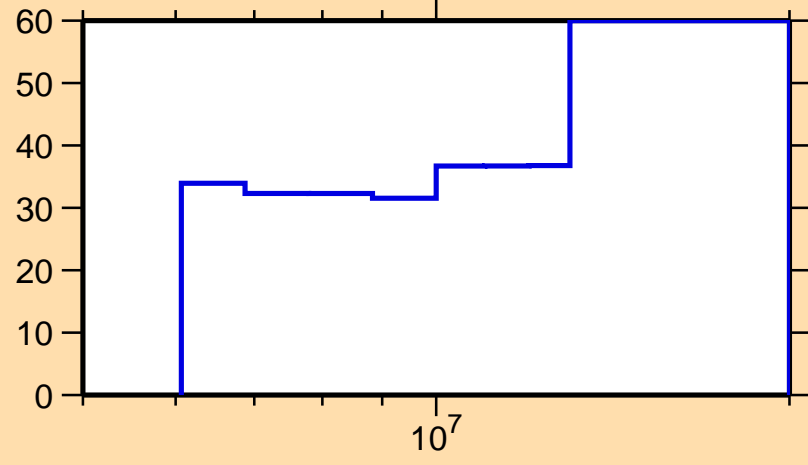
\Delta\sigma/\sigma vs. E for ^{171}\text{Dy}(n,2n)
