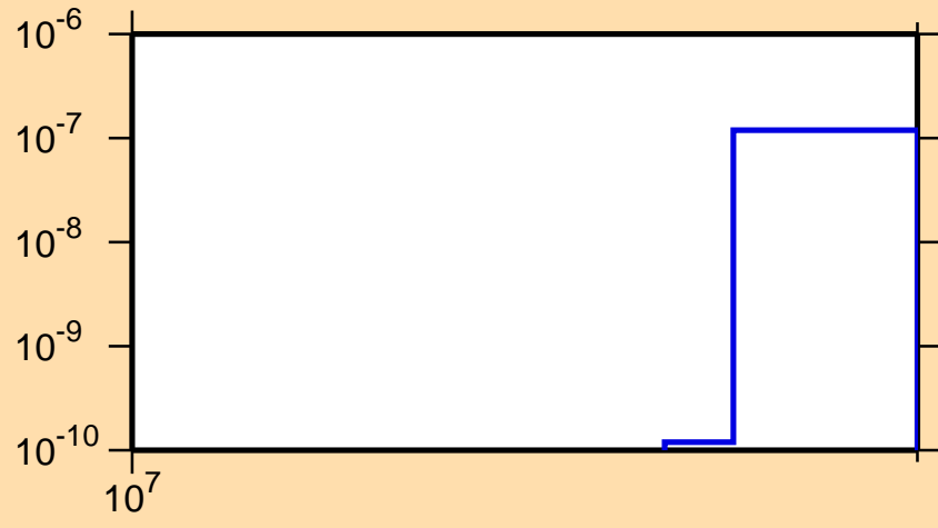
\sigma vs. E for ^{171}\text{Dy}(n,\text{nd})
