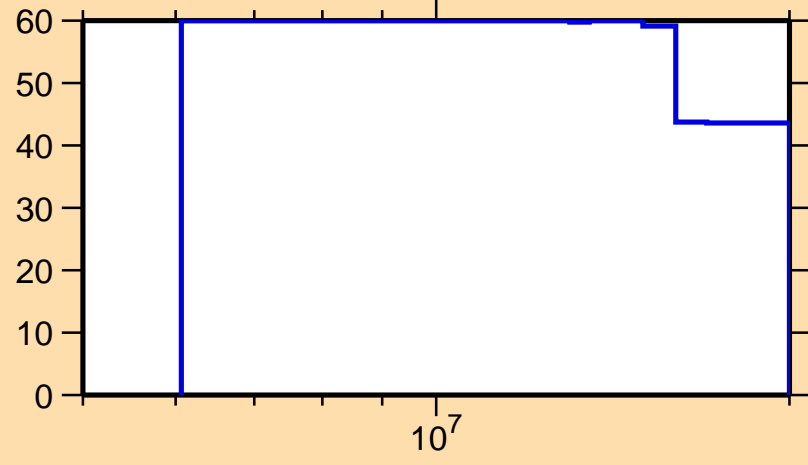
\Delta\sigma/\sigma vs. E for ^{171}\text{Dy}(n,\text{inel.})
