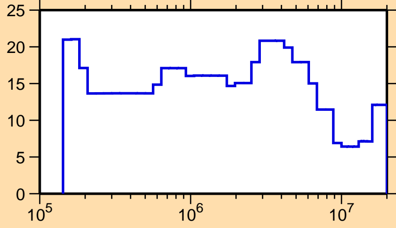
\Delta\sigma/\sigma vs. E for ^{171}\text{Dy}(n,\text{el.})
