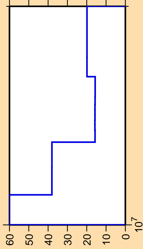
\Delta\sigma/\sigma vs. E for ^{171}\text{Dy}(n,3n)
