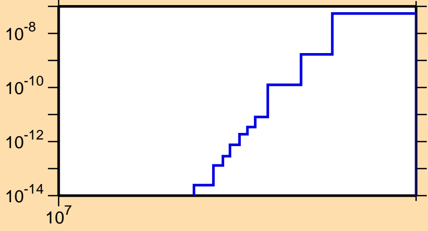
\sigma vs. E for ^{171}\text{Dy}(n,2n\alpha)
