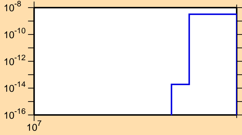
\sigma vs. E for ^{171}\text{Dy}(n,2np)
