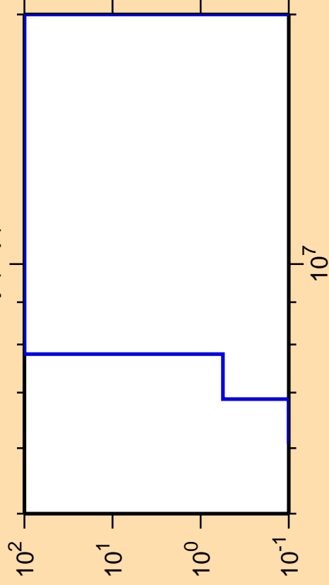
\Delta\sigma/\sigma vs. E for ^{171}\text{Dy}(n,p)
