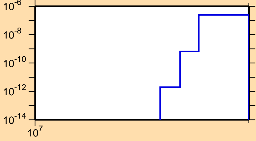
\sigma vs. E for ^{171}\text{Dy}(n,nt)
