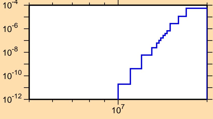
\sigma vs. E for ^{171}\text{Dy}(n,n\alpha)
