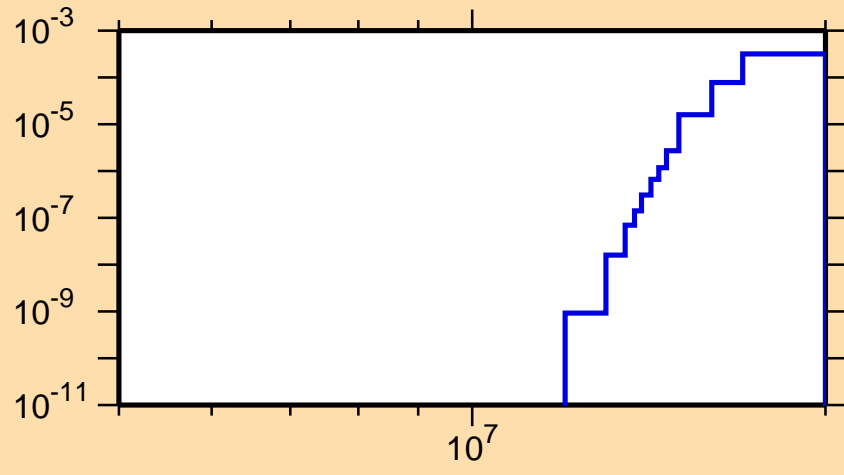
\sigma vs. E for ^{171}\text{Dy}(n,d)
