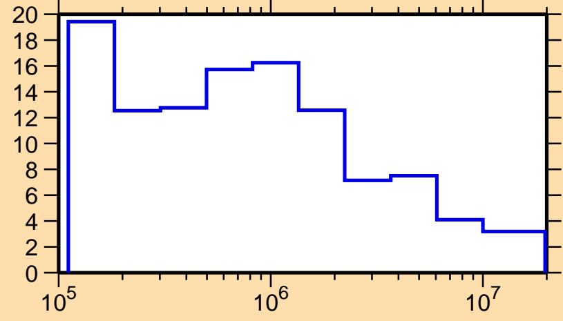
\Delta\sigma/\sigma vs. E for ^{171}\text{Dy}(n,\text{tot.})
