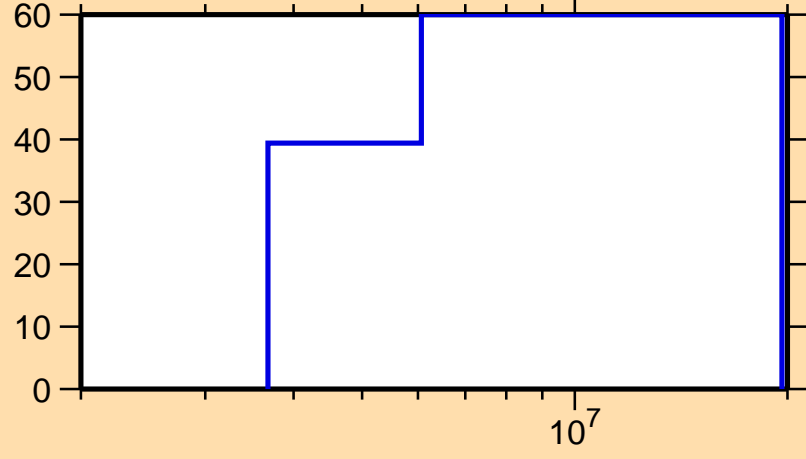
\Delta\sigma/\sigma vs. E for ^{171}\text{Dy}(n,n\text{cont.})
