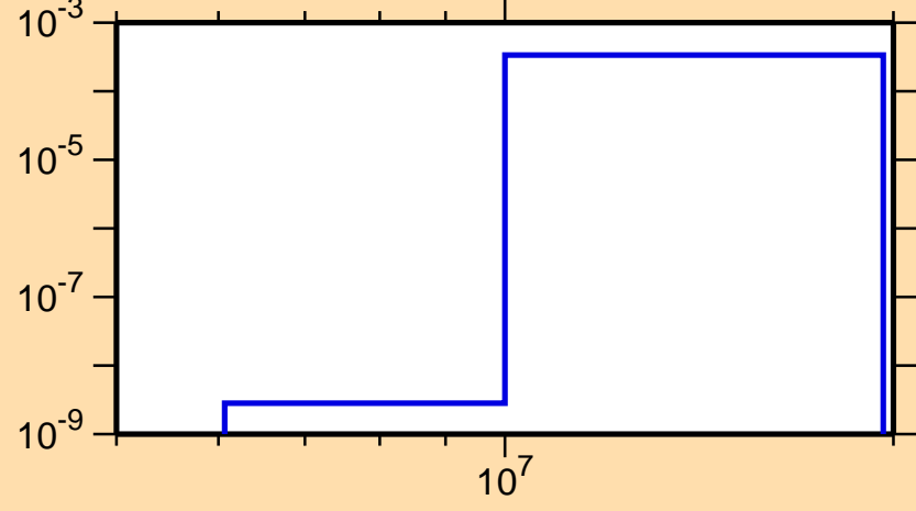
\sigma vs. E for ^{171}\text{Dy}(n,p)
