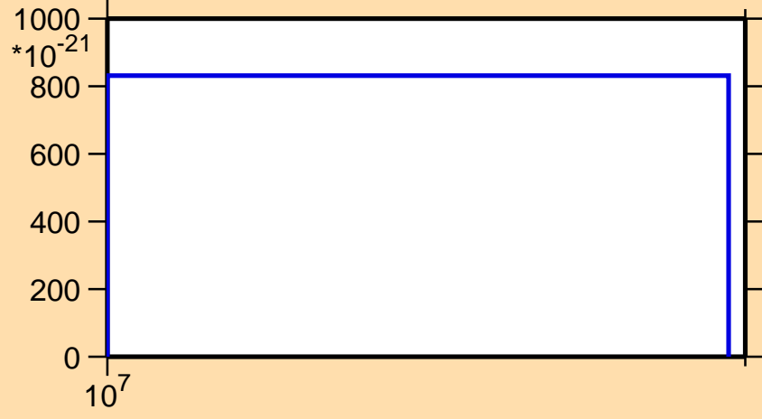
\sigma vs. E for ^{171}\text{Dy} (mt 11)
