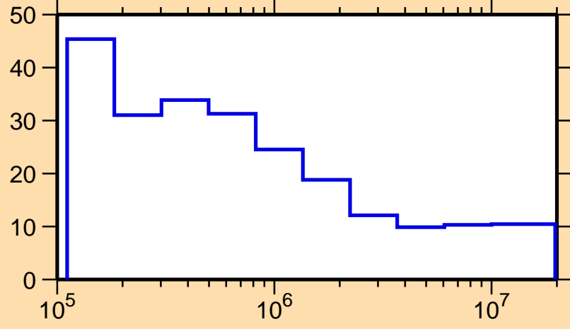
\Delta\sigma/\sigma vs. E for ^{171}\text{Dy}(n,n\text{onel.})
