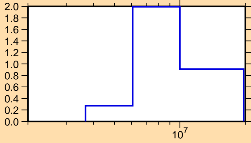
\sigma vs. E for ^{171}\text{Dy}(n,2n)
