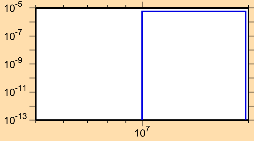
\sigma vs. E for ^{171}\text{Dy}(n,t)
