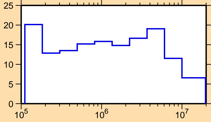
\Delta\sigma/\sigma vs. E for ^{171}\text{Dy}(n,el.)
