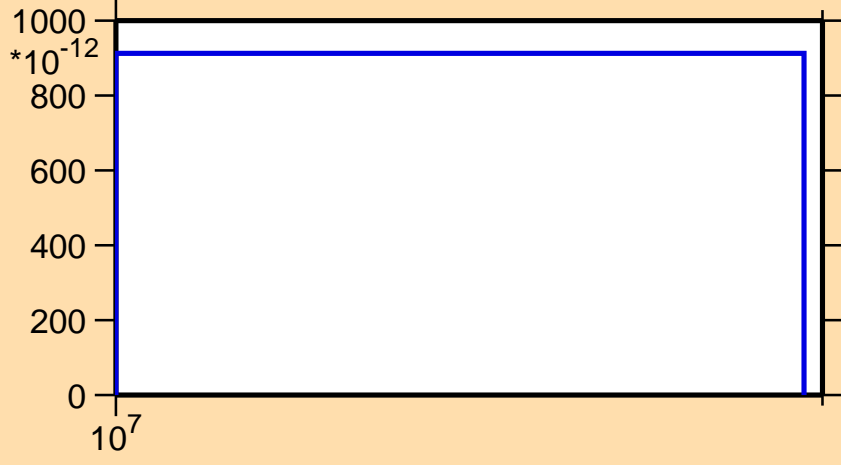
\sigma vs. E for ^{171}\text{Dy}(n,nd)
