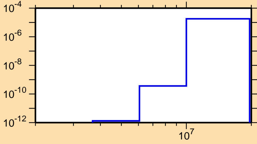
\sigma vs. E for ^{171}\text{Dy}(n,\alpha)
