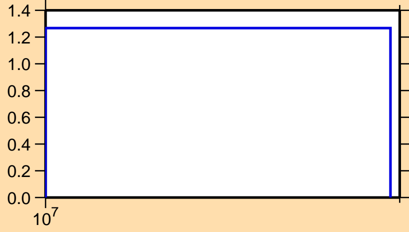
\sigma vs. E for ^{171}\text{Dy}(n,3n)
