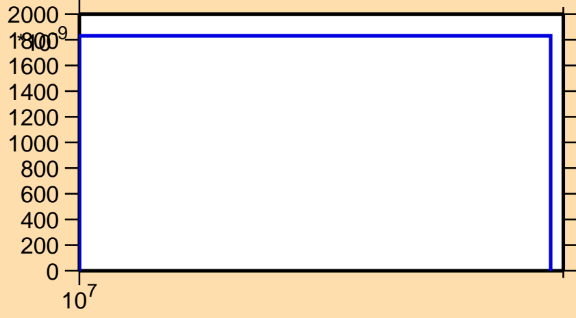
\sigma vs. E for ^{171}\text{Dy}(n,np)
