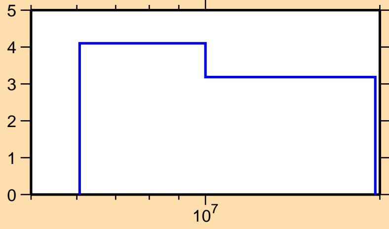
\Delta\sigma/\sigma vs. E for ^{171}\text{Dy}(n,\text{tot.})
