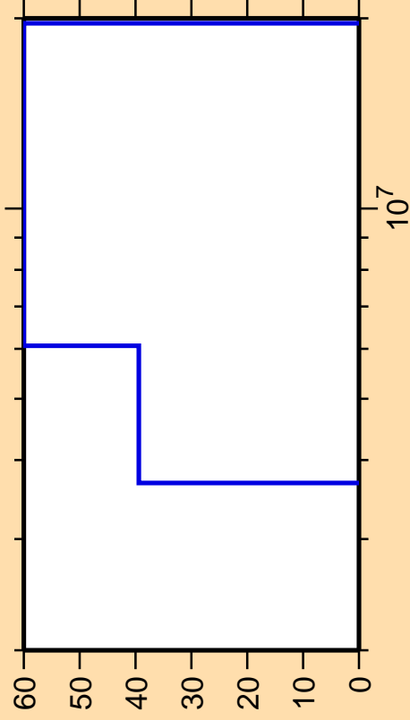
\Delta\sigma/\sigma vs. E for ^{171}\text{Dy}(n,n\text{cont.})
