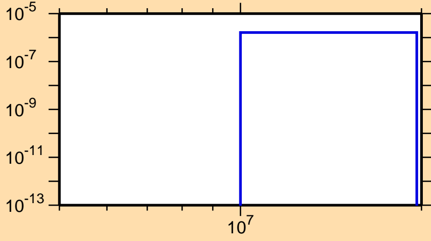
\sigma vs. E for ^{171}\text{Dy}(n,n\alpha)
