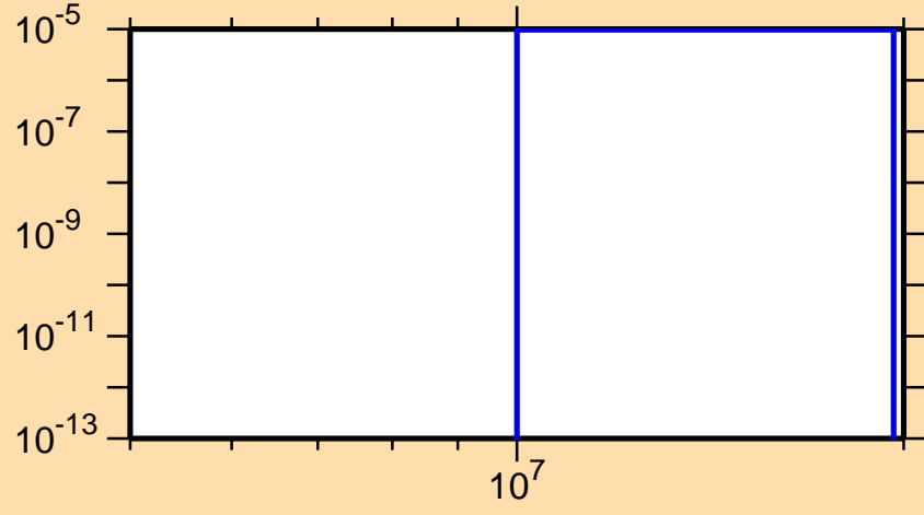
\sigma vs. E for ^{171}\text{Dy}(n,d)
