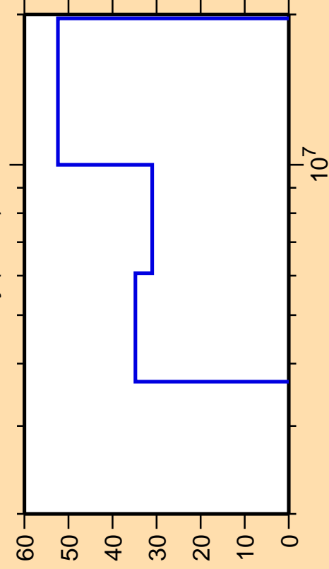
\Delta\sigma/\sigma vs. E for ^{171}\text{Dy}(n,2n)
