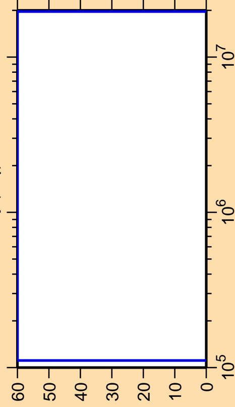
\Delta\sigma/\sigma vs. E for ^{171}\text{Dy}(n,\gamma)
