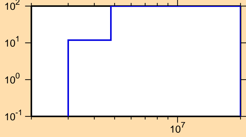
\Delta\sigma/\sigma vs. E for ^{171}\text{Dy}(n,n\text{cont.})
