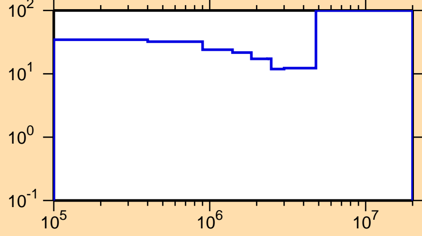
\Delta\sigma/\sigma vs. E for ^{171}\text{Dy}(n,\text{inel.})
