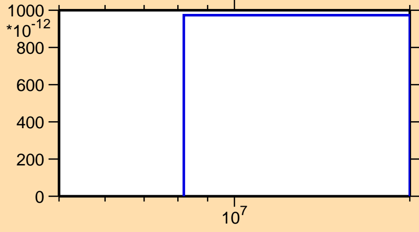
\sigma vs. E for ^{171}\text{Dy}(n,\text{nd})
