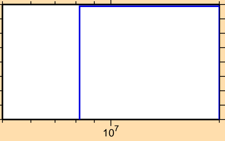
\sigma vs. E for ^{171}\text{Dy}(n,d)
