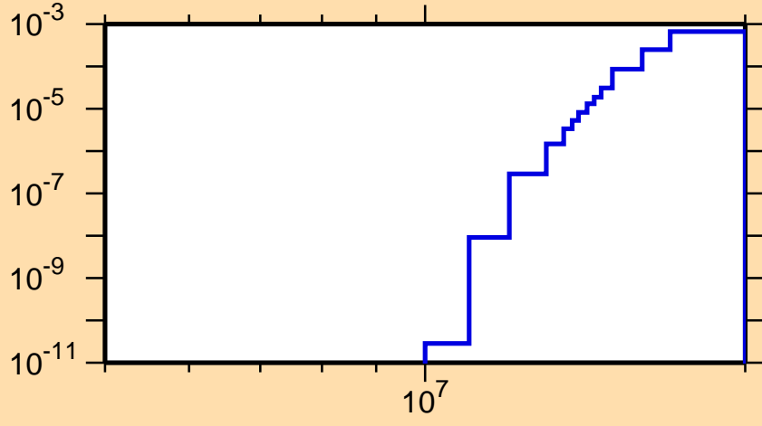
\sigma vs. E for ^{172}\text{Dy}(n,p)
