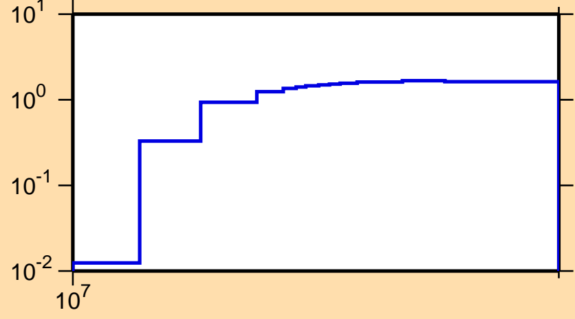
\sigma vs. E for ^{172}\text{Dy}(n,3n)
