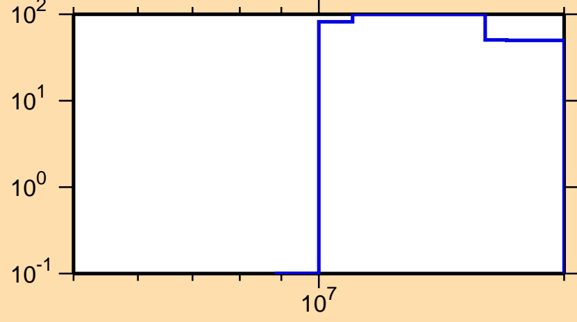
\Delta\sigma/\sigma vs. E for ^{172}\text{Dy}(n,p)
