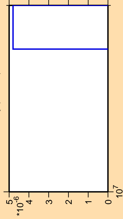
\Delta\sigma/\sigma vs. E for ^{172}\text{Dy} (mt 11)
