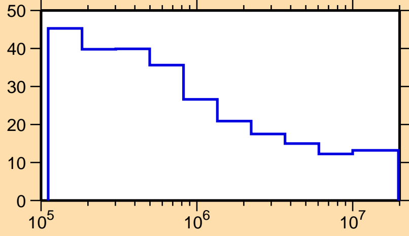
\Delta\sigma/\sigma vs. E for ^{172}\text{Dy}(n,nonel.)
