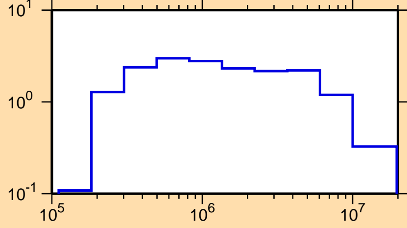
\sigma vs. E for ^{172}\text{Dy}(n,\text{inel.})
