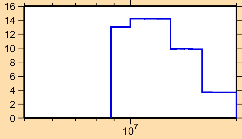
\Delta\sigma/\sigma vs. E for ^{173}\text{Dy}(n,el.)
