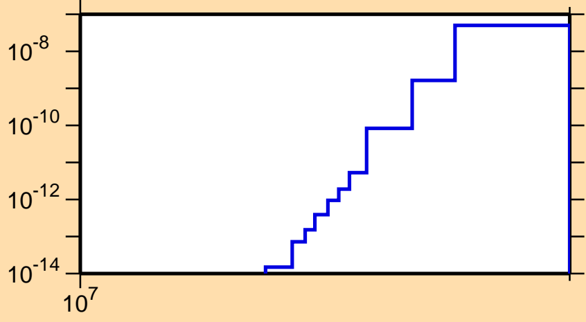
\sigma vs. E for ^{173}\text{Dy}(n,2n\alpha)
