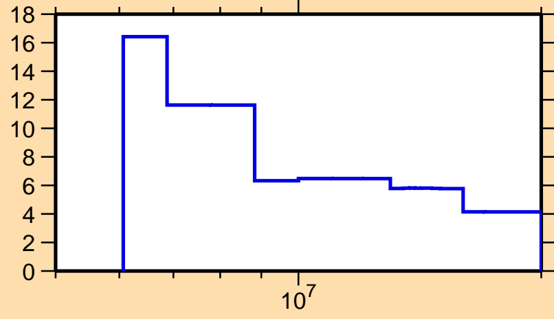
\Delta\sigma/\sigma vs. E for ^{173}\text{Dy}(n,\text{tot.})
