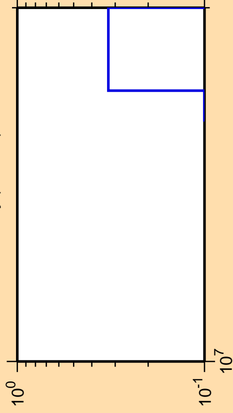
\Delta\sigma/\sigma vs. E for ^{173}\text{Dy}(n,3n\alpha)
