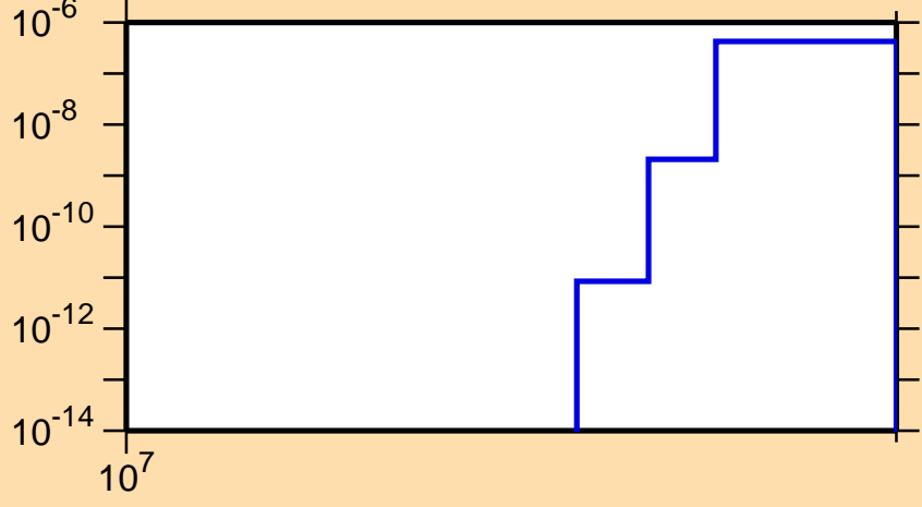
\sigma vs. E for ^{173}\text{Dy}(n,nt)
