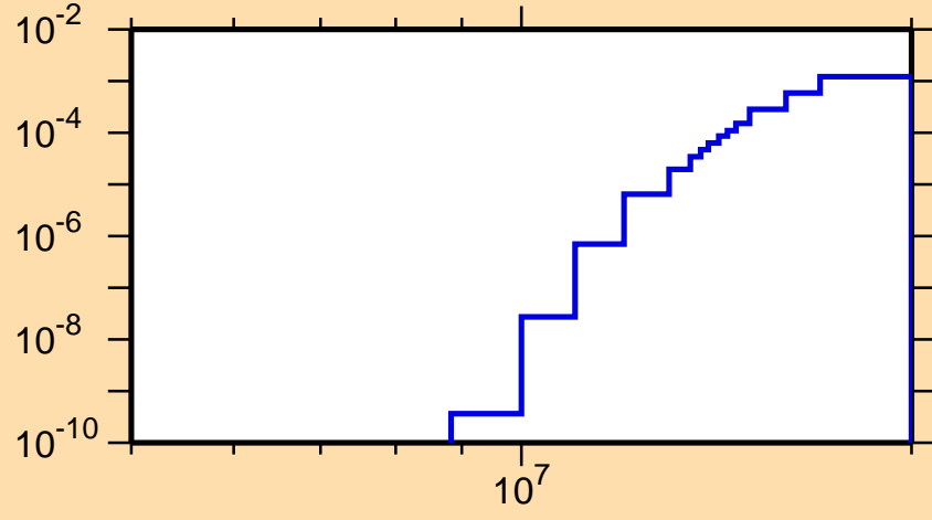
\sigma vs. E for ^{173}\text{Dy}(n,p)
