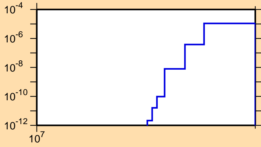
\sigma vs. E for ^{173}\text{Dy}(n,np)
