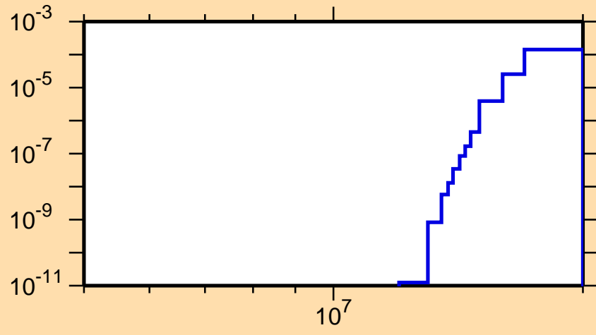
\sigma vs. E for ^{173}\text{Dy}(n,d)
