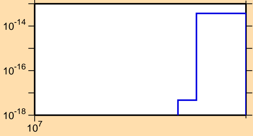
\sigma vs. E for ^{173}\text{Dy}(n,3n\alpha)
