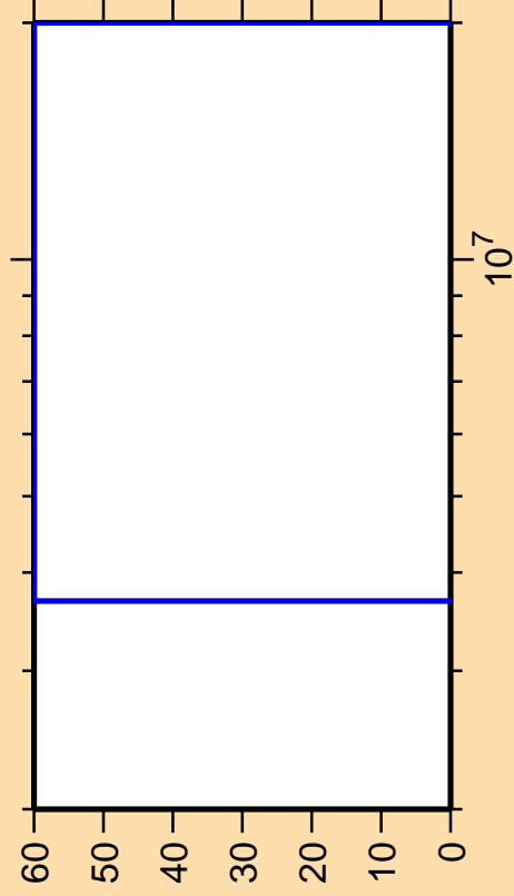
\Delta\sigma/\sigma vs. E for ^{173}\text{Dy}(n,\gamma)
