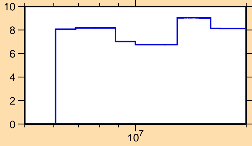
\Delta\sigma/\sigma vs. E for ^{173}\text{Dy}(n,\text{nonel.})
