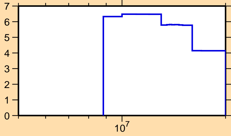
\Delta\sigma/\sigma vs. E for ^{173}\text{Dy}(n,\text{tot.})
