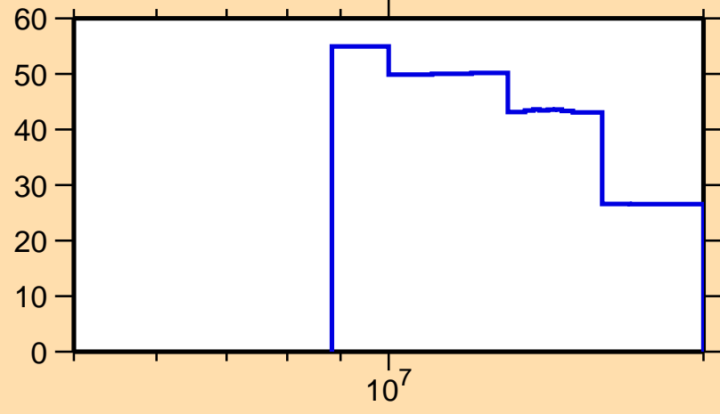
\Delta\sigma/\sigma vs. E for ^{173}\text{Dy}(n,n_1)
