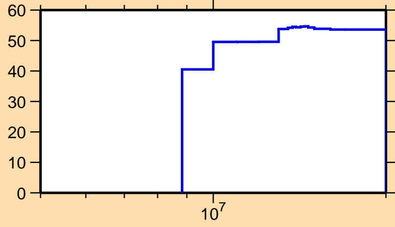
\Delta\sigma/\sigma vs. E for ^{173}\text{Dy}(n,2n)
