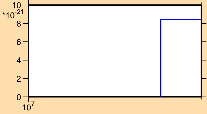
\sigma vs. E for ^{173}\text{Dy} (mt 11)
