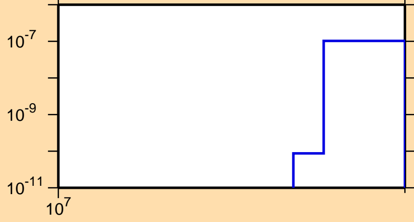
\sigma vs. E for ^{173}\text{Dy}(n,\text{nd})
