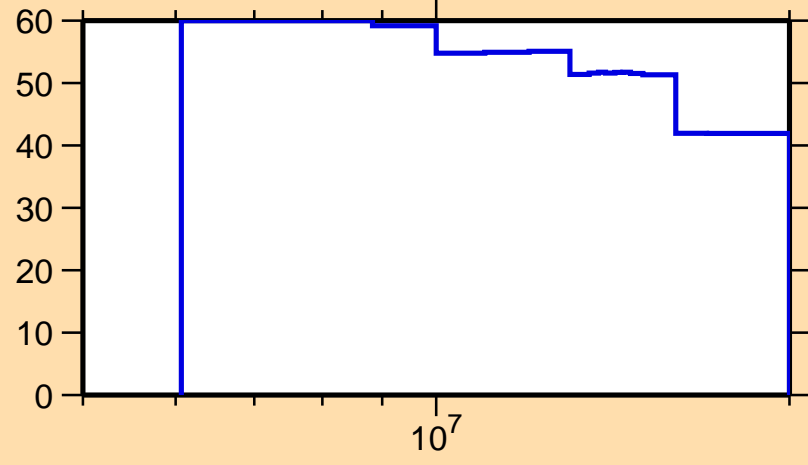
\Delta\sigma/\sigma vs. E for ^{173}\text{Dy}(n,\text{inel.})
