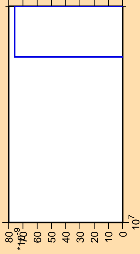
\Delta\sigma/\sigma vs. E for ^{173}\text{Dy} (mt 11)
