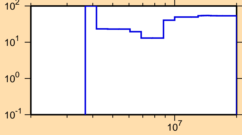
\Delta\sigma/\sigma vs. E for ^{173}\text{Dy}(n,2n)
