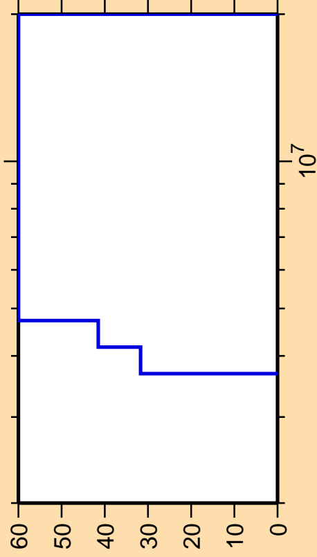
\Delta\sigma/\sigma vs. E for ^{173}\text{Dy}(n,n\text{cont.})
