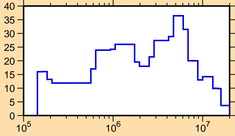
\Delta\sigma/\sigma vs. E for ^{173}\text{Dy}(n,\text{el.})
