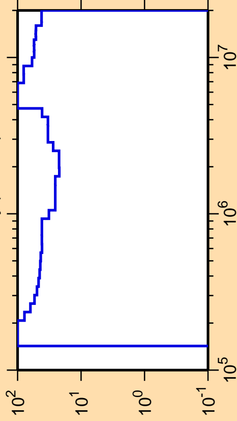
\Delta\sigma/\sigma vs. E for ^{173}\text{Dy}(n,\text{inel.})
