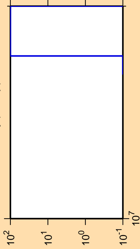
\Delta\sigma/\sigma vs. E for ^{173}\text{Dy}(n,2np)
