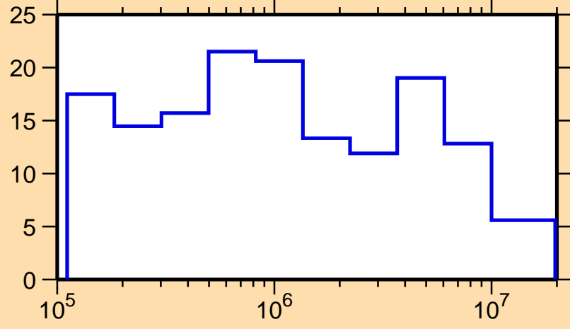
\Delta\sigma/\sigma vs. E for ^{173}\text{Dy}(n, tot.)
