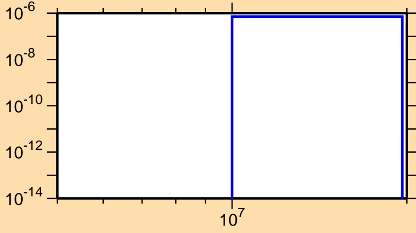
\sigma vs. E for ^{173}\text{Dy}(n,n\alpha)
