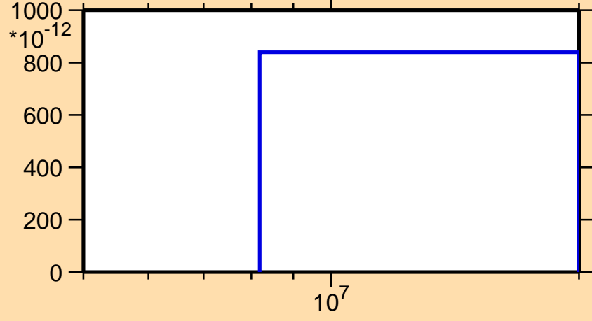
\sigma vs. E for ^{173}\text{Dy}(n,\text{nd})
