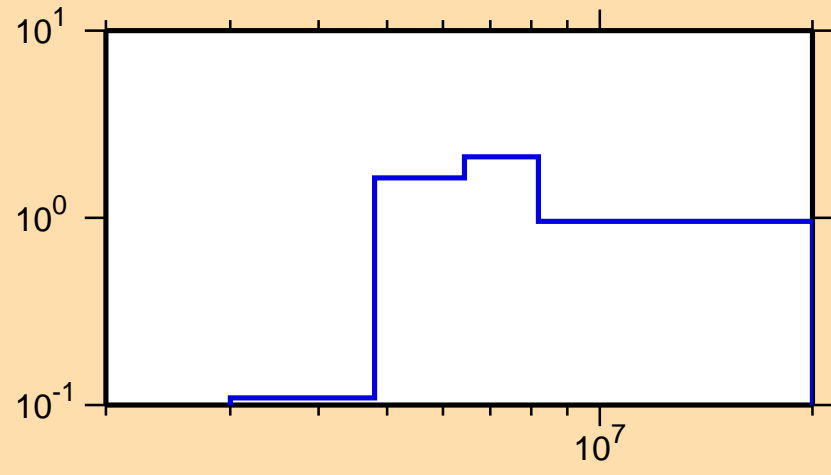
\sigma vs. E for ^{173}\text{Dy}(n,2n)
