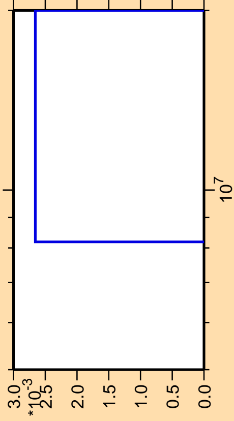
\Delta\sigma/\sigma vs. E for ^{173}\text{Dy}(n,3n\alpha)
