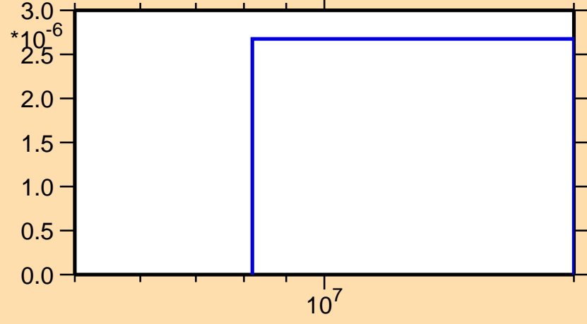
\sigma vs. E for ^{173}\text{Dy}(n,d)
