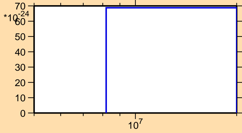
\sigma vs. E for ^{173}\text{Dy}(\text{mt } 11)
