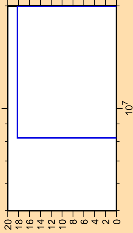
\Delta\sigma/\sigma vs. E for ^{173}\text{Dy}(n,3n)
