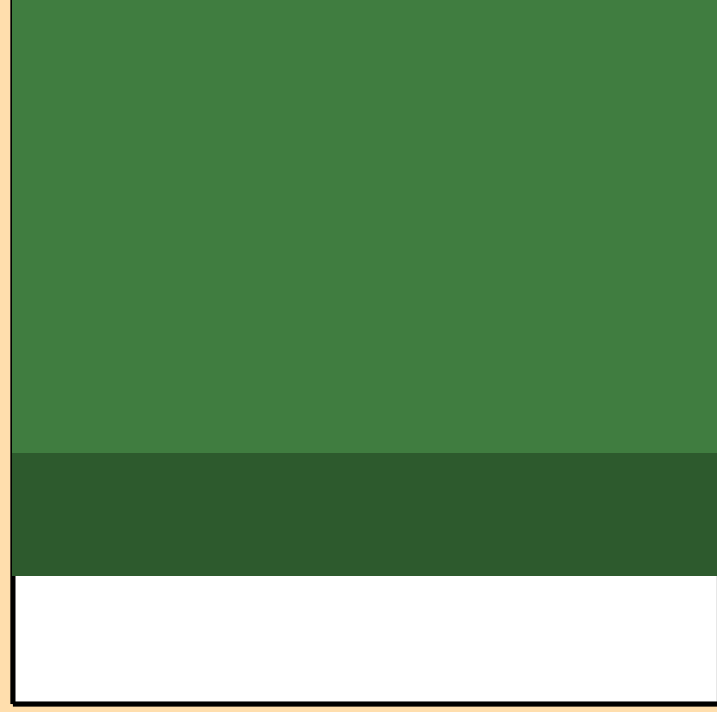
\Delta\sigma/\sigma vs. E for ^{173}\text{Dy}(n,n_1)
