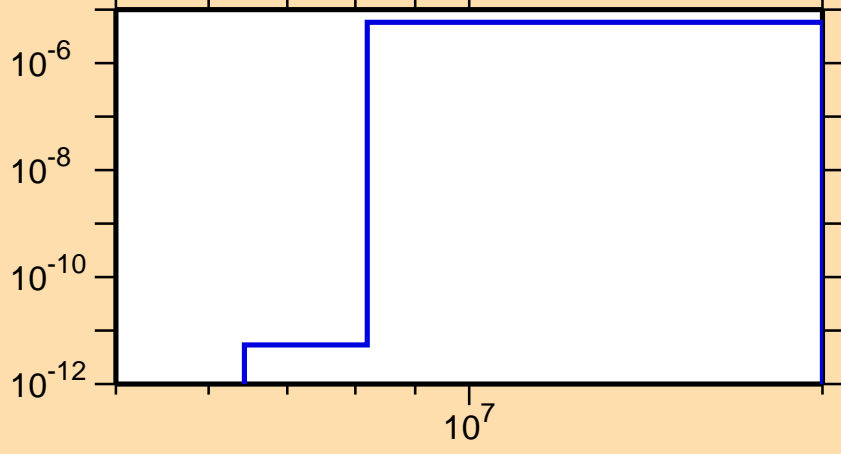
\sigma vs. E for ^{173}\text{Dy}(n,\alpha)
