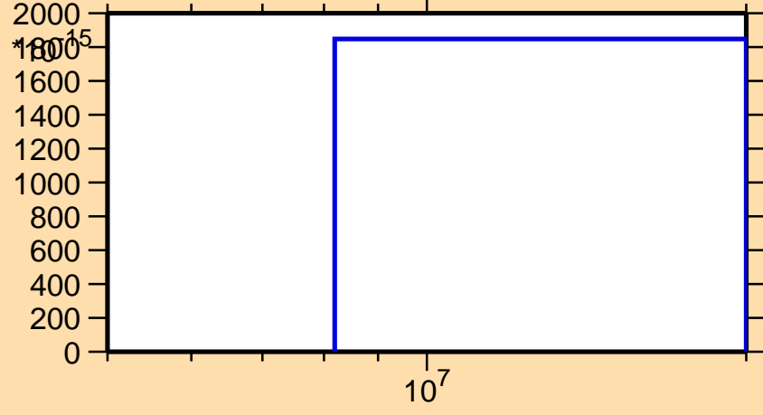
\sigma vs. E for ^{173}\text{Dy}(n,2np)
