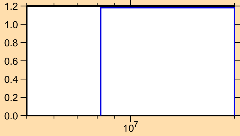
\sigma vs. E for ^{173}\text{Dy}(n,3n)
