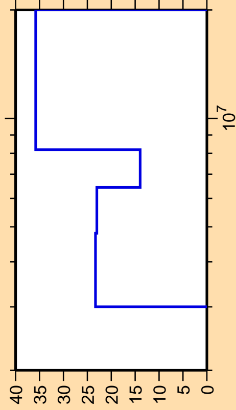
\Delta\sigma/\sigma vs. E for ^{173}\text{Dy}(n,2n)
