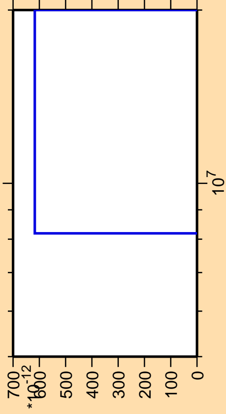
\Delta\sigma/\sigma vs. E for ^{173}\text{Dy}(\text{mt } 11)
