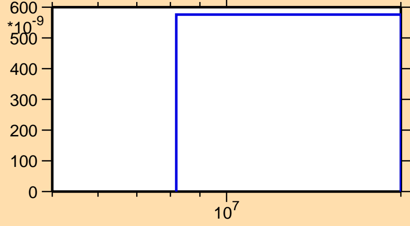
\sigma vs. E for ^{173}\text{Dy}(n,n\alpha)
