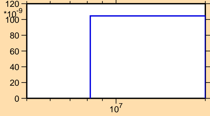
\sigma vs. E for ^{173}\text{Dy}(n,np)
