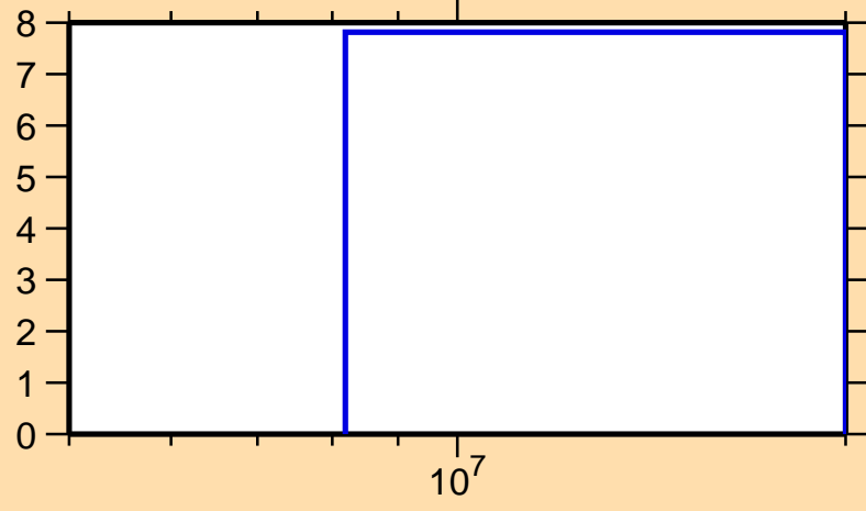
\Delta\sigma/\sigma vs. E for ^{173}\text{Dy}(n,\text{nonel.})
