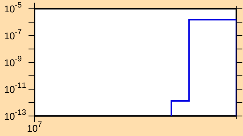
\sigma vs. E for ^{146}\text{Er}(n,2np)
