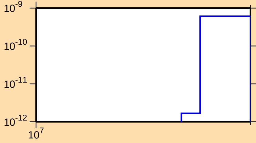
\sigma vs. E for ^{146}\text{Er}(n,2n\alpha)
