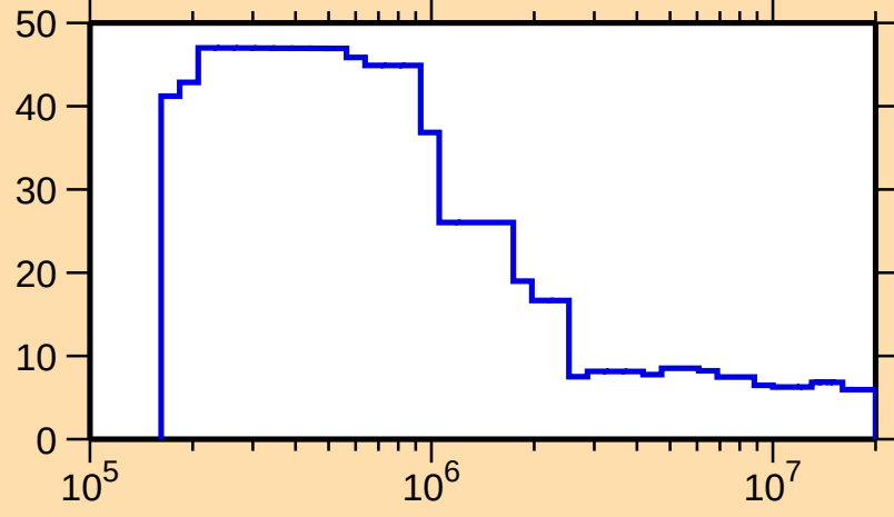
\Delta\sigma/\sigma vs. E for ^{146}\text{Er}(n,\text{nonel.})
