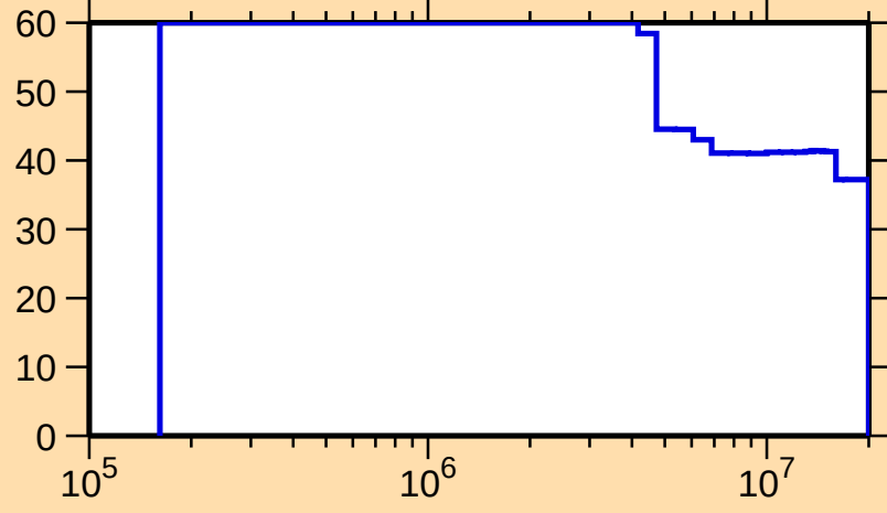
\Delta\sigma/\sigma vs. E for ^{146}\text{Er}(n,n\text{cont.})
