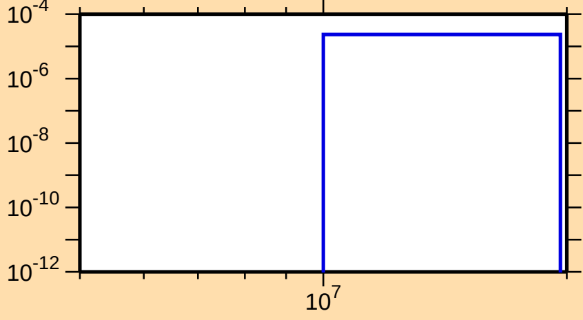
\sigma vs. E for ^{146}\text{Er}(n,t)
