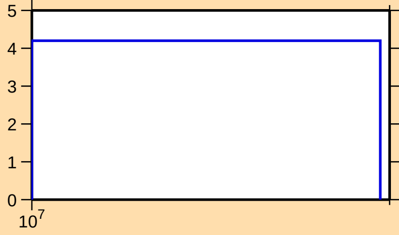
\Delta\sigma/\sigma vs. E for ^{146}\text{Er}(n,\text{tot.})
