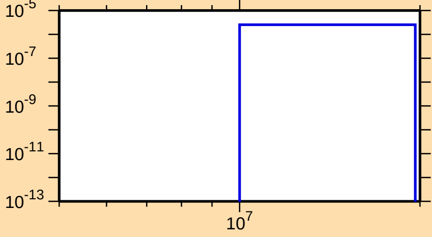
\sigma vs. E for ^{146}\text{Er}(n,\text{pt})
