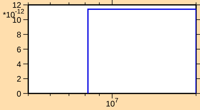
\sigma vs. E for ^{146}\text{Er}(\text{mt } 34)
