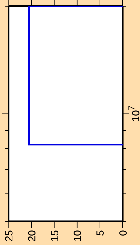
\Delta\sigma/\sigma vs. E for ^{146}\text{Er}(n,\text{nd})
