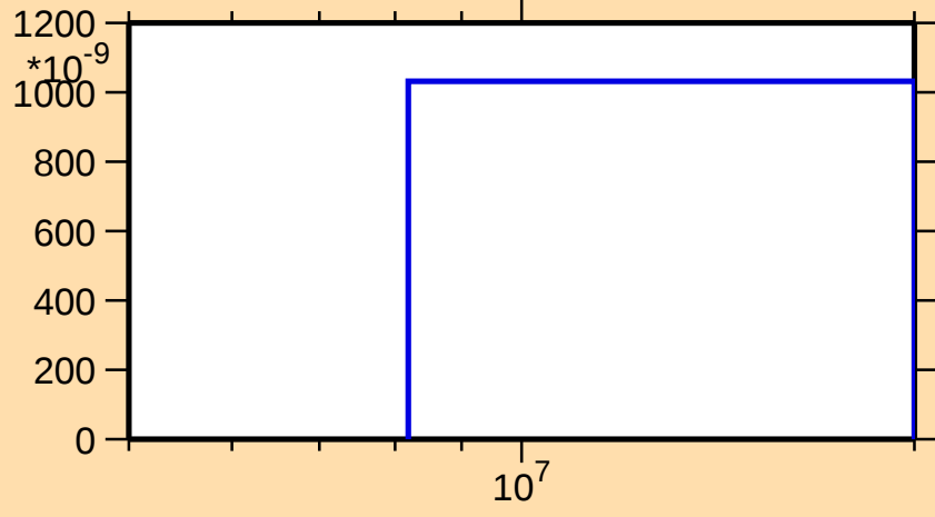
\sigma vs. E for ^{146}\text{Er}(\text{mt } 45)
