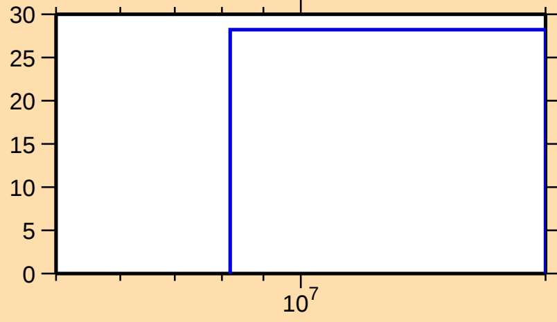
\Delta\sigma/\sigma vs. E for ^{146}\text{Er}(n,\text{inel.})
