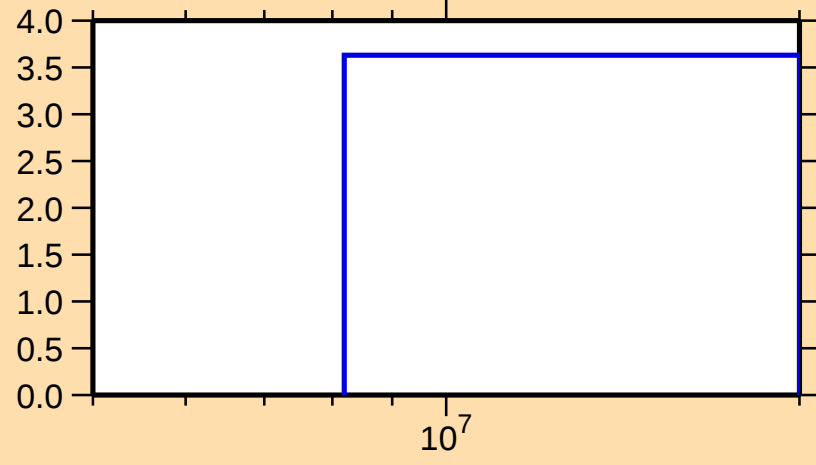
\Delta\sigma/\sigma vs. E for ^{146}\text{Er}(n,\text{tot.})
