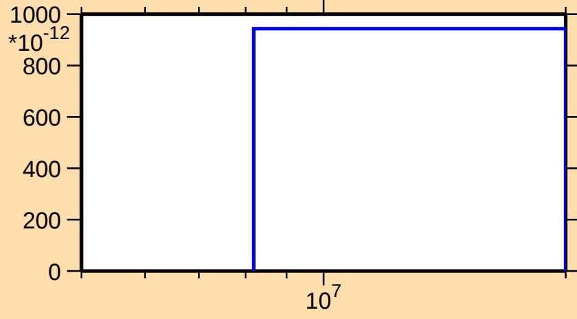
\sigma vs. E for ^{146}\text{Er}(\text{mt117})
