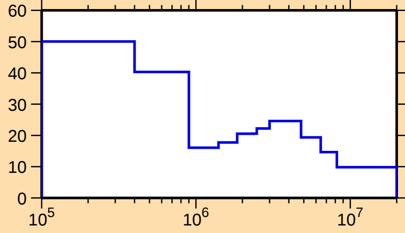
\Delta\sigma/\sigma vs. E for ^{146}\text{Er}(n,\text{el.})
