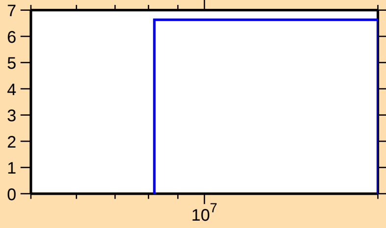
\Delta\sigma/\sigma vs. E for ^{146}\text{Er}(n,\text{nonel.})
