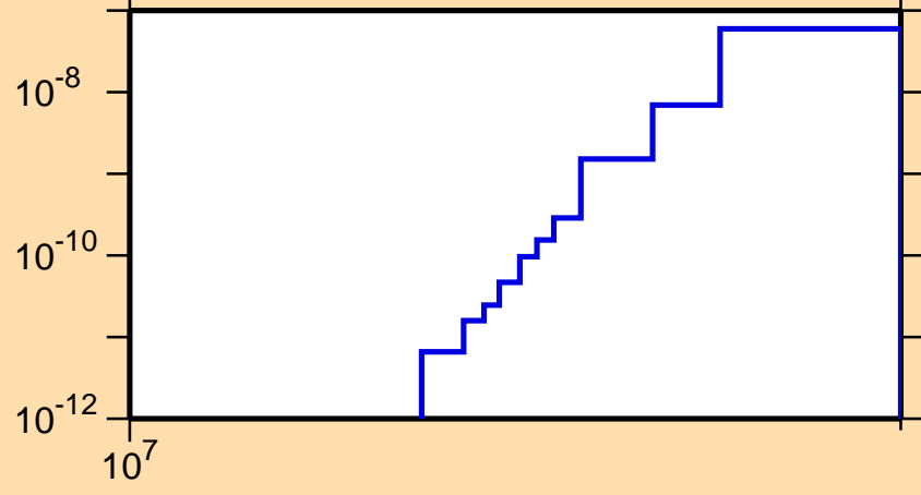
\sigma vs. E for ^{147}\text{Er}(\text{mt } 34)
