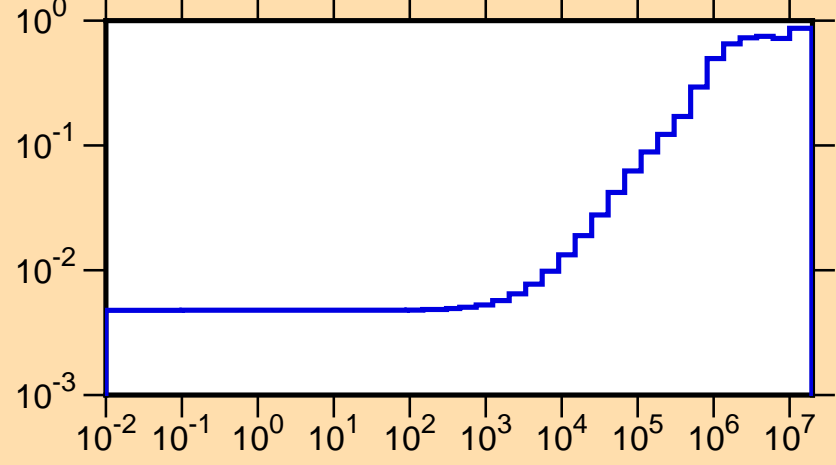
\mu vs. E for ^{147}\text{Er}(\text{mt251})
