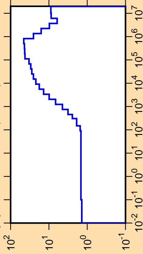
\Delta\mu/\mu vs. E for ^{147}\text{Er}(\text{mt251})
