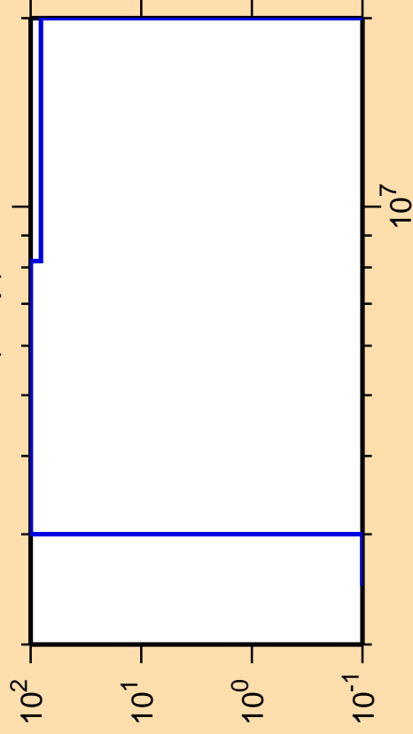
\Delta\sigma/\sigma vs. E for ^{147}\text{Er}(n,np)
