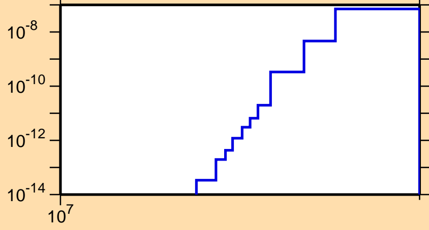
\sigma vs. E for ^{147}\text{Er}(n,2n\alpha)
