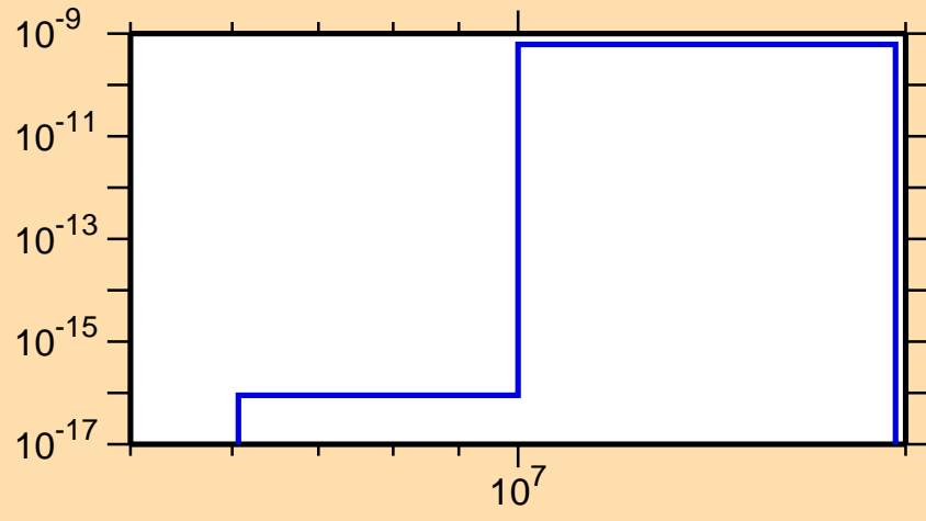
\sigma vs. E for ^{147}\text{Er}(\text{mt117})
