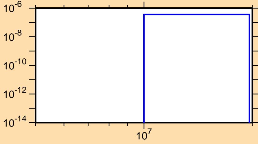
\sigma vs. E for ^{147}\text{Er}(\text{mt } 45)
