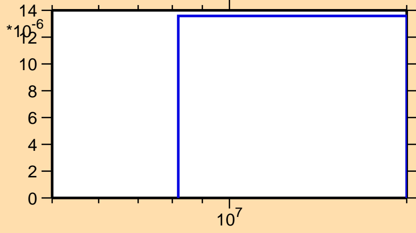
\sigma vs. E for ^{147}\text{Er}(n,\text{pt})
