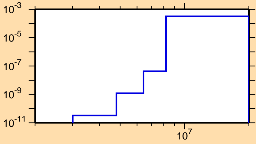
\sigma vs. E for ^{147}\text{Er}(n,\text{He3})
