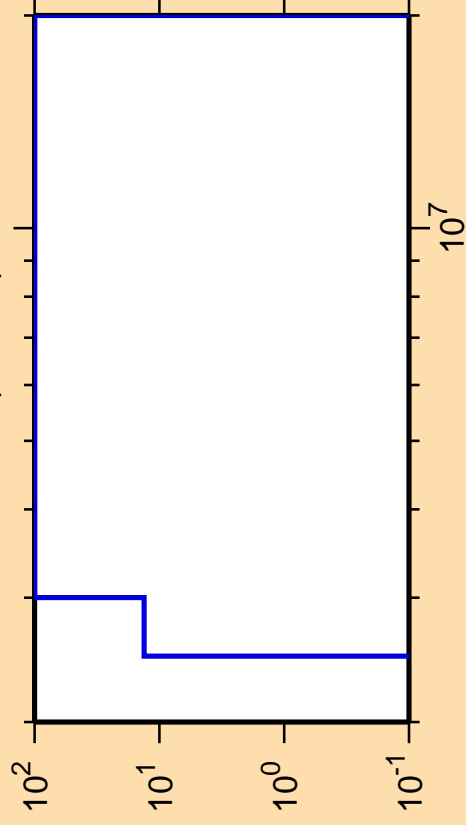
\Delta\sigma/\sigma vs. E for ^{147}\text{Er}(n,\text{He3})
