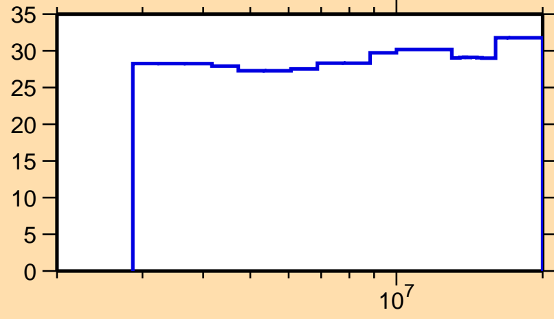
\Delta\sigma/\sigma vs. E for ^{148}\text{Er}(n,n\text{onel.})
