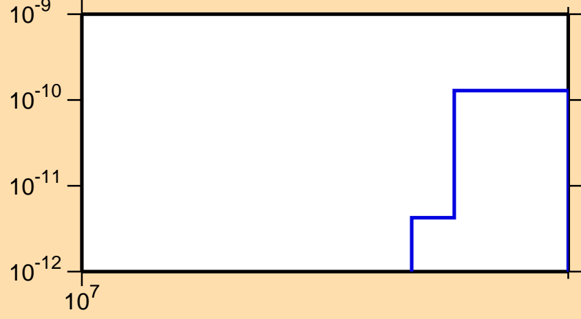
\sigma vs. E for ^{148}\text{Er}(\text{mt } 34)
