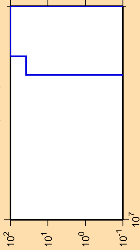
\Delta\sigma/\sigma vs. E for ^{148}\text{Er}(\text{mt } 34)
