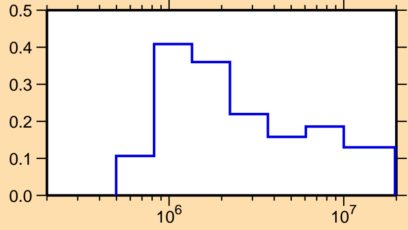
\sigma vs. E for ^{148}\text{Er}(n,\text{inel.})
