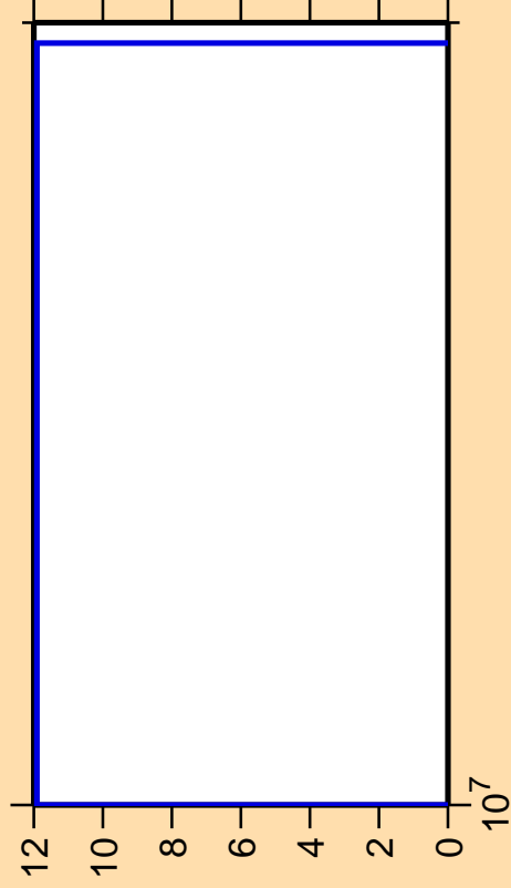
\Delta\sigma/\sigma vs. E for ^{148}\text{Er} (mt 34)
