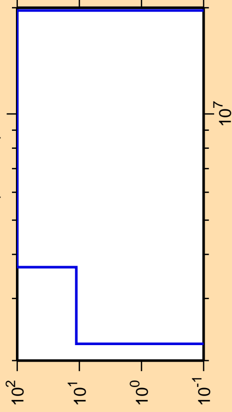
\Delta\sigma/\sigma vs. E for ^{148}\text{Er}(n,\text{He3})
