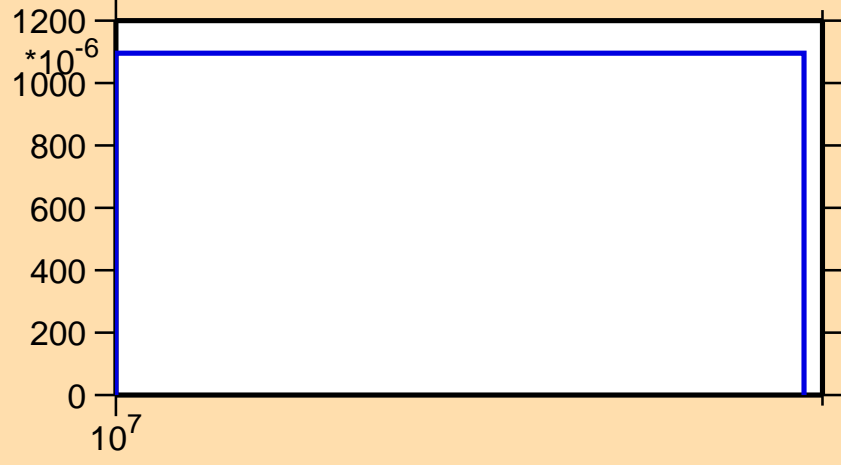
\sigma vs. E for ^{148}\text{Er}(n,2n)
