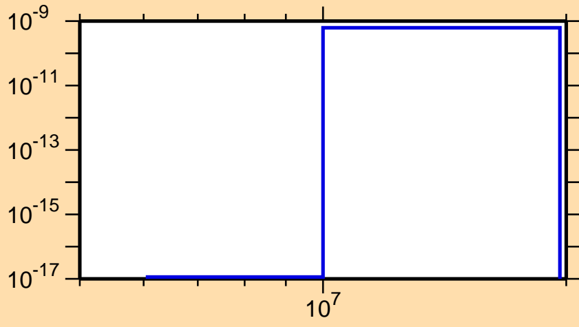
\sigma vs. E for ^{148}\text{Er}(\text{mt117})
