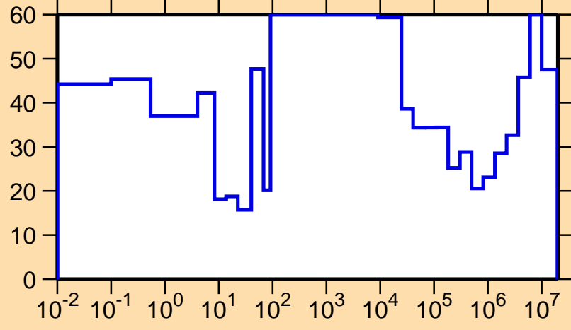
\Delta\sigma/\sigma vs. E for ^{148}\text{Er}(n,\text{el.})
