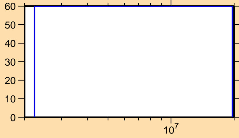
\Delta\sigma/\sigma vs. E for ^{148}\text{Er}(n,n\text{cont.})
