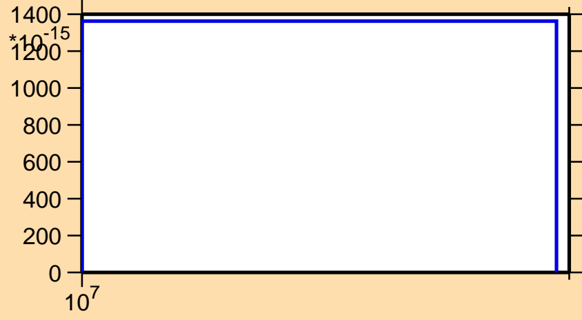
\sigma vs. E for ^{148}\text{Er} (mt 34)
