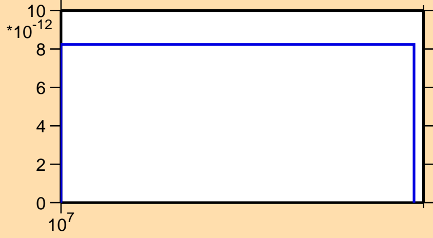
\sigma vs. E for ^{148}\text{Er}(n,\text{nd})
