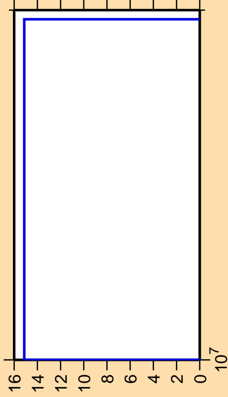
\Delta\sigma/\sigma vs. E for ^{148}\text{Er}(n,2n\alpha)
