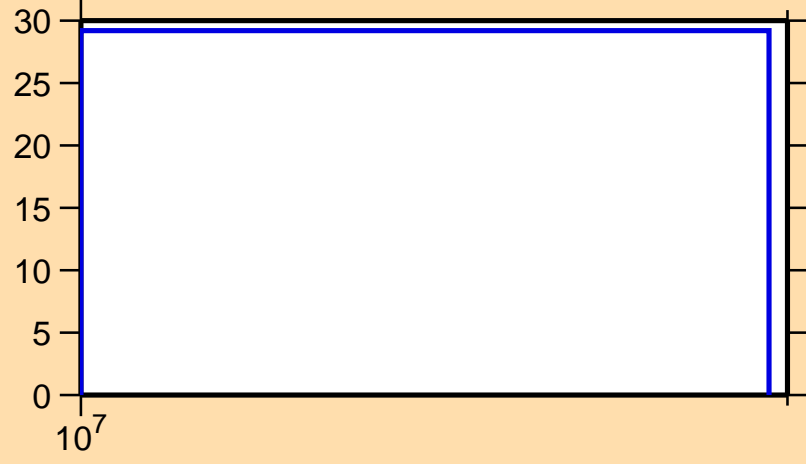
\Delta\sigma/\sigma vs. E for ^{148}\text{Er}(n,\text{tot.})
