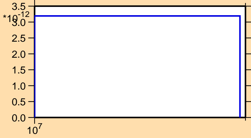
\sigma vs. E for ^{148}\text{Er}(n,2n\alpha)
