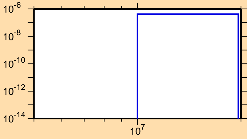
\sigma vs. E for ^{148}\text{Er}(\text{mt } 45)
