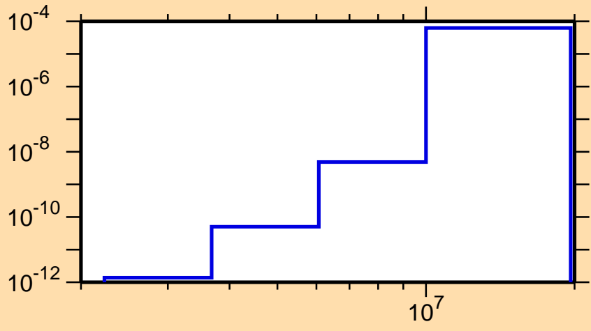
\sigma vs. E for ^{148}\text{Er}(n,\text{He3})
