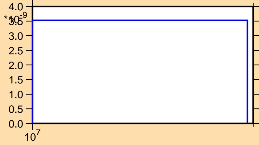
\sigma vs. E for ^{148}\text{Er}(n,2np)
