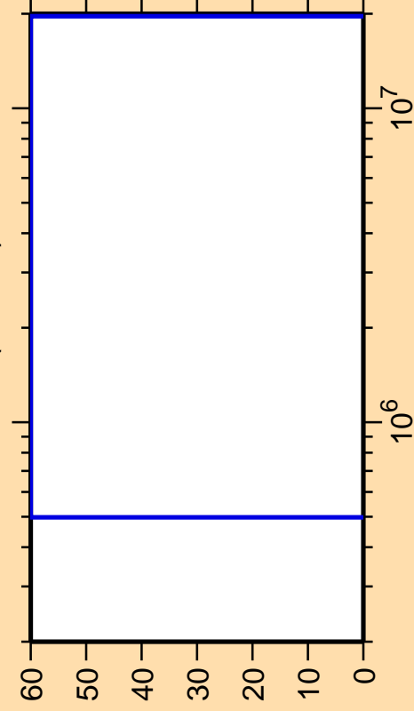
\Delta\sigma/\sigma vs. E for ^{148}\text{Er}(n,\text{inel.})
