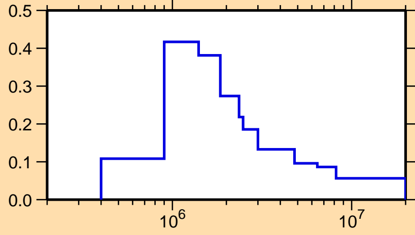
\sigma vs. E for ^{148}\text{Er}(n,n_1)
