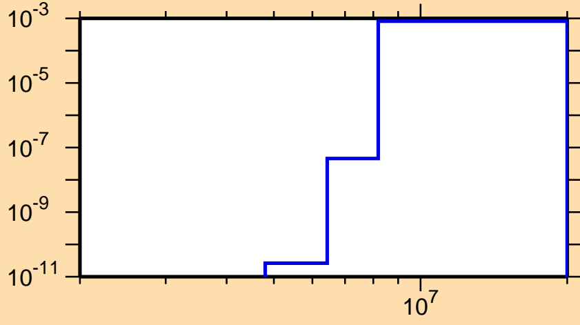
\sigma vs. E for ^{148}\text{Er}(n,pd)
