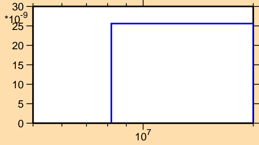
\sigma vs. E for ^{148}\text{Er}(n,\text{pt})
