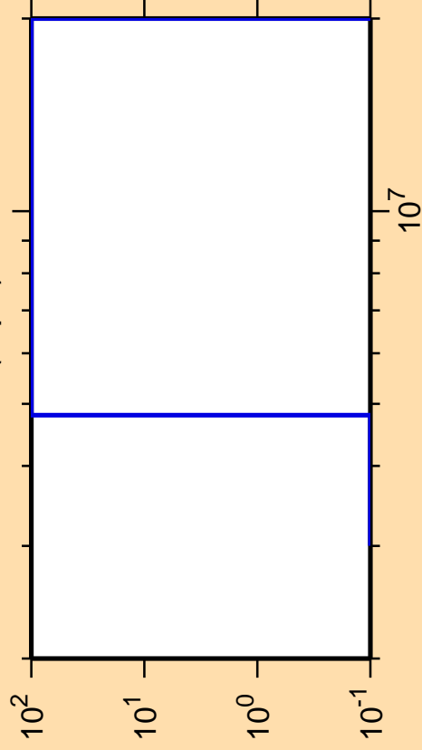
\Delta\sigma/\sigma vs. E for ^{148}\text{Er}(n,pd)
