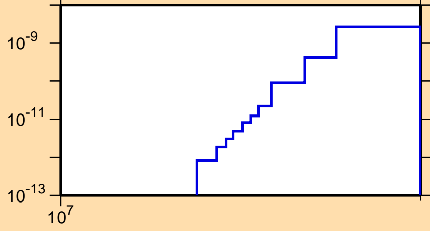
\sigma vs. E for ^{149}\text{Er}(\text{mt117})
