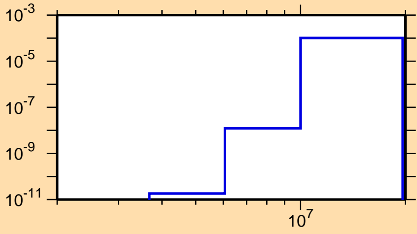
\sigma vs. E for ^{149}\text{Er}(n,\text{He3})
