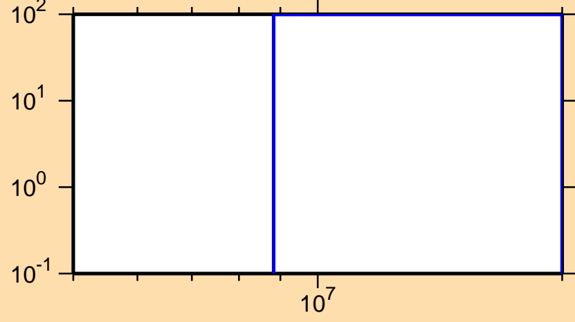
\Delta\sigma/\sigma vs. E for ^{149}\text{Er}(n,2n)
