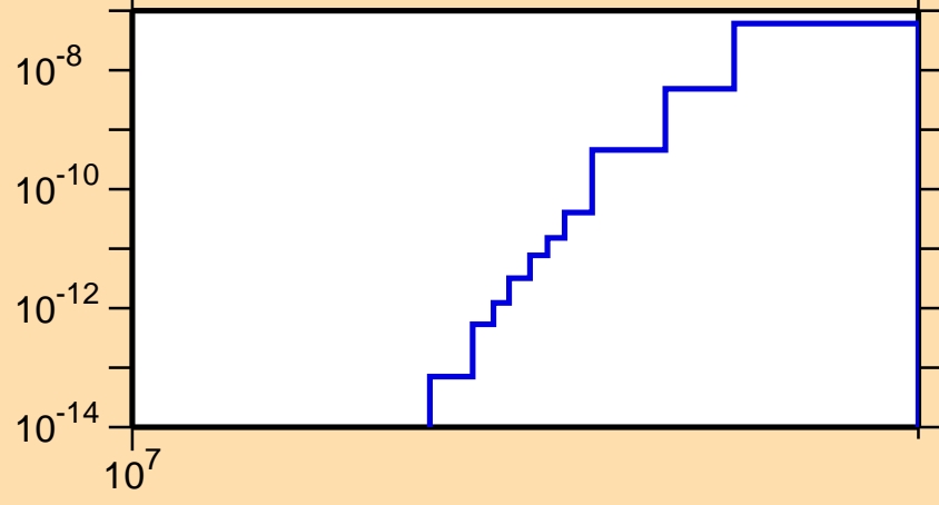
\sigma vs. E for ^{149}\text{Er}(n,2n\alpha)
