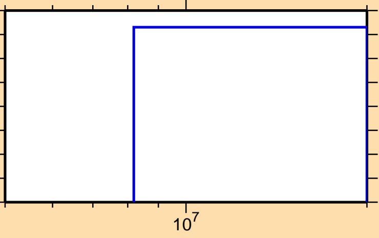
\sigma vs. E for ^{149}\text{Er}(n,\text{pt})
