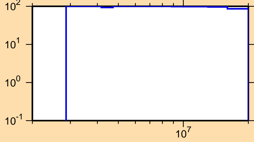
\Delta\sigma/\sigma vs. E for ^{150}\text{Er}(n,ncont.)
