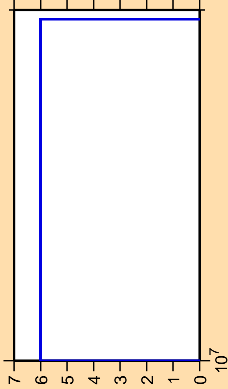
\Delta\sigma/\sigma vs. E for ^{150}\text{Er}(n,2n\alpha)
