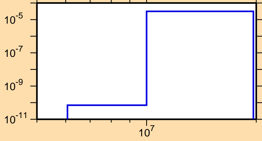
\sigma vs. E for ^{150}\text{Er}(n,\text{pd})
