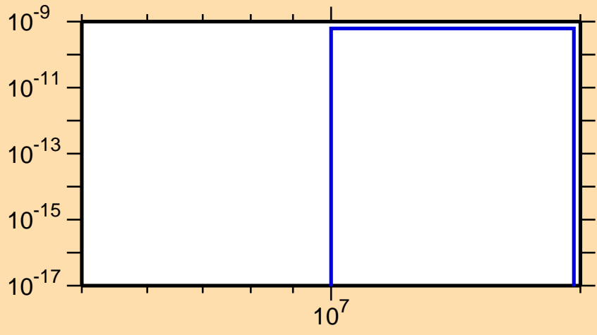
\sigma vs. E for ^{150}\text{Er}(\text{mt117})
