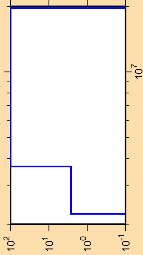
\Delta\sigma/\sigma vs. E for ^{150}\text{Er}(n,\text{He3})
