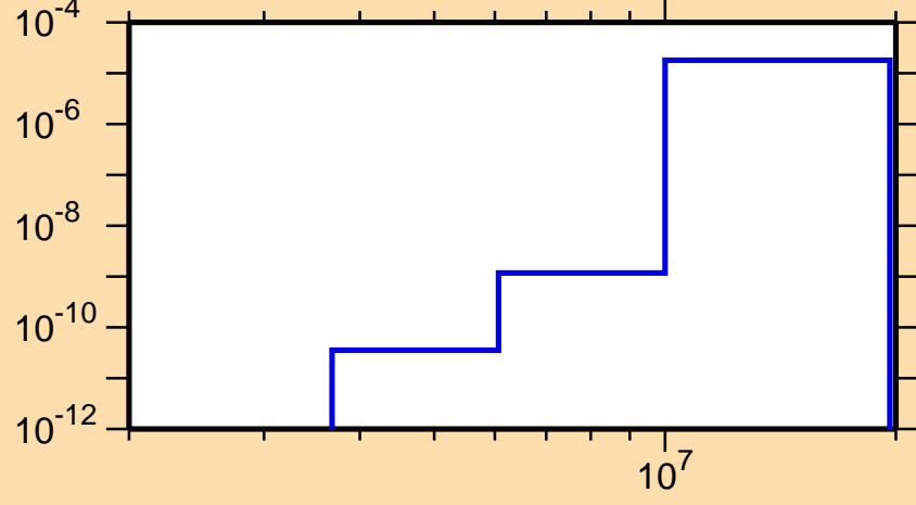
\sigma vs. E for ^{150}\text{Er}(n,\text{He3})
