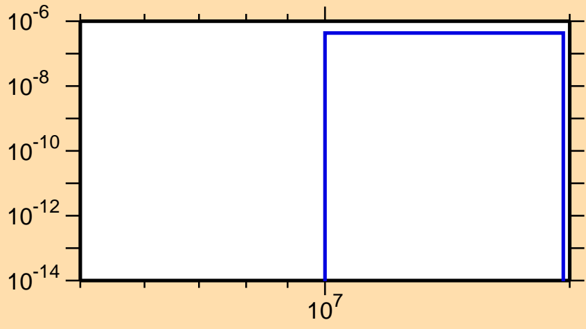
\sigma vs. E for ^{150}\text{Er} (mt 45)
