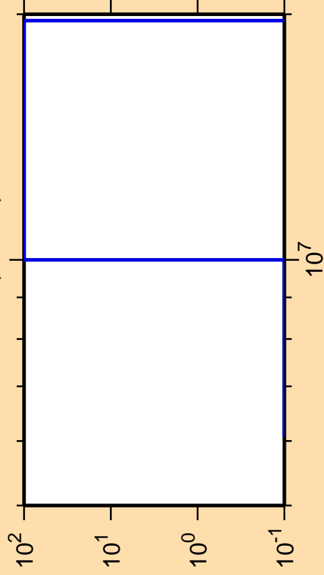
\Delta\sigma/\sigma vs. E for ^{150}\text{Er} (mt 45)
