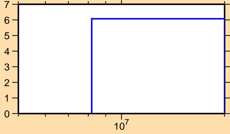
\Delta\sigma/\sigma vs. E for ^{150}\text{Er}(n,\text{tot.})
