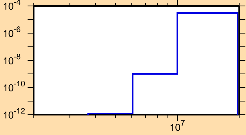
\sigma vs. E for ^{151}\text{Er}(n,\text{He3})
