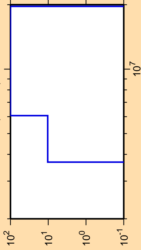
\Delta\sigma/\sigma vs. E for ^{151}\text{Er}(n,\text{He3})
