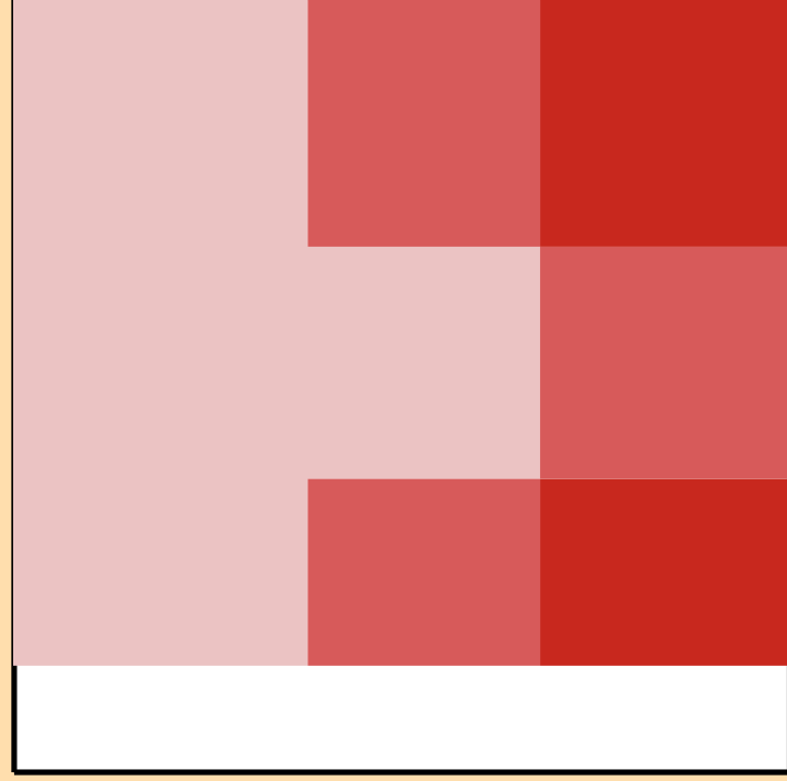
\Delta\sigma/\sigma vs. E for ^{152}\text{Er}(n,\text{nonel.})
