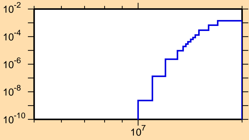
\sigma vs. E for ^{152}\text{Er}(n,t)
