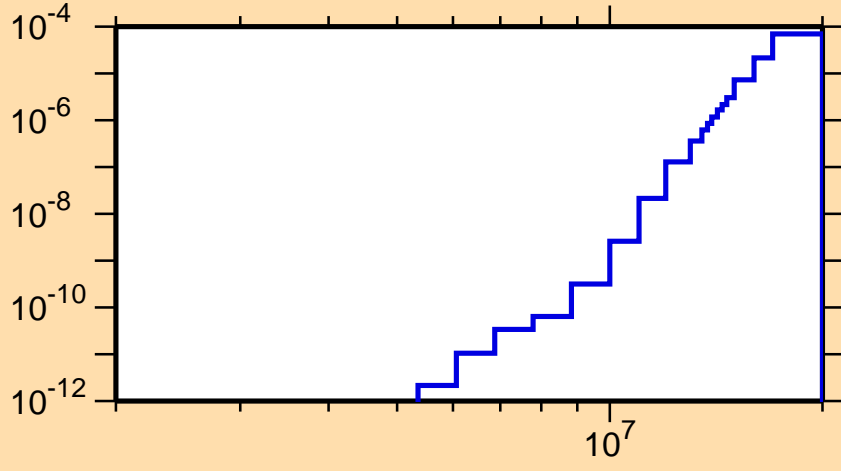
\sigma vs. E for ^{152}\text{Er}(n,\text{He3})
