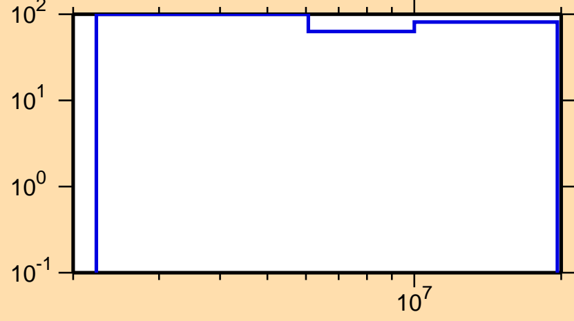
\Delta\sigma/\sigma vs. E for ^{152}\text{Er}(n,n\text{cont.})
