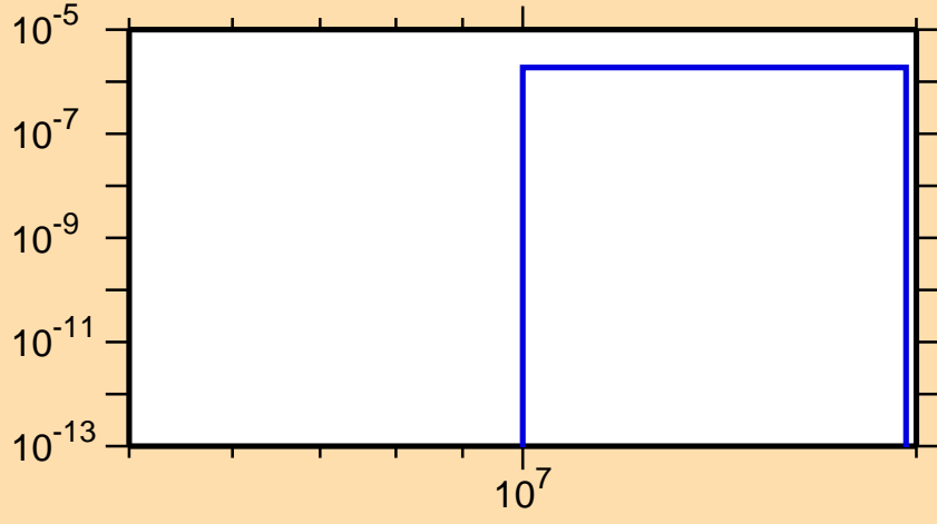
\sigma vs. E for ^{152}\text{Er}(n,\text{pd})
