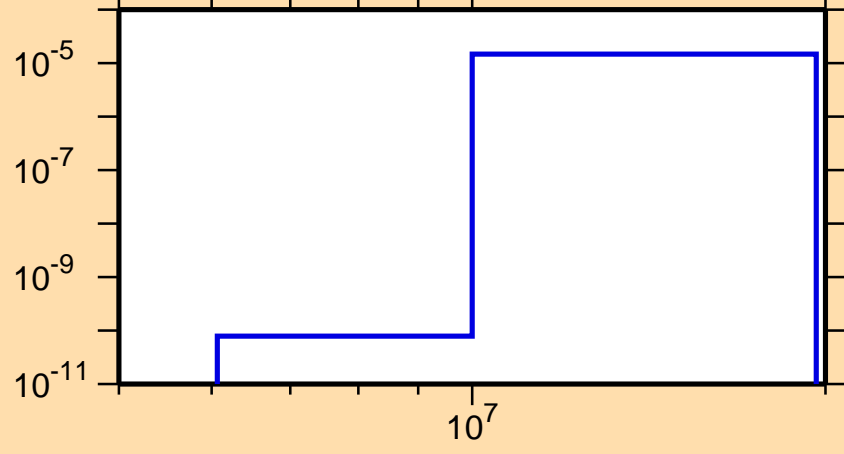
\sigma vs. E for ^{152}\text{Er}(\text{mt } 45)
