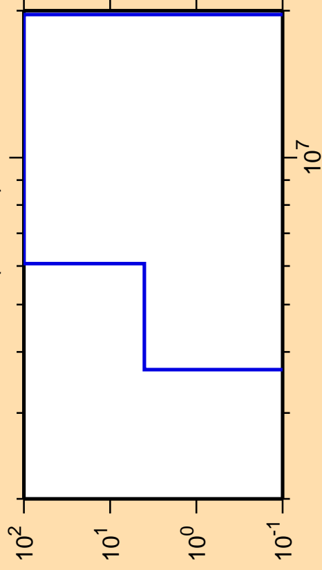
\Delta\sigma/\sigma vs. E for ^{152}\text{Er}(n,\text{He3})
