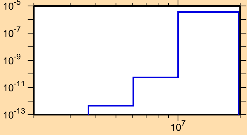
\sigma vs. E for ^{152}\text{Er}(n,\text{He3})
