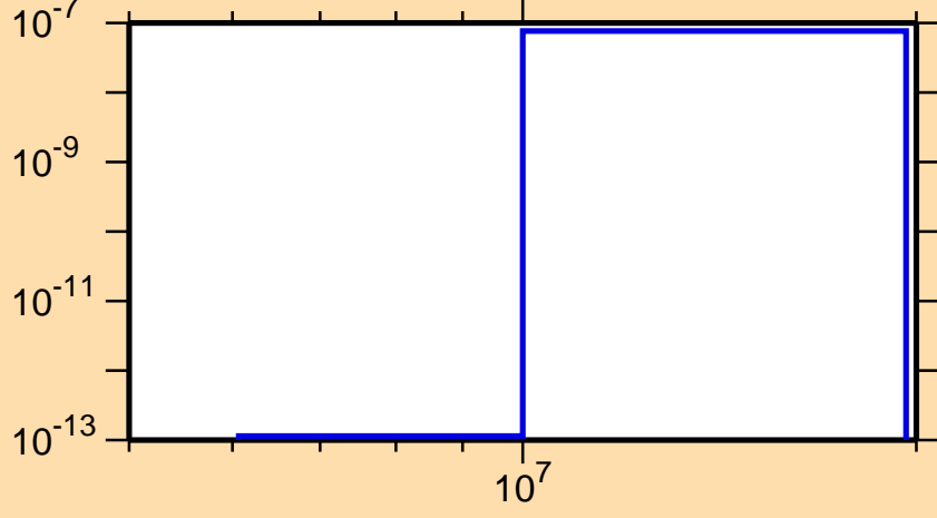
\sigma vs. E for ^{152}\text{Er}(\text{mt117})
