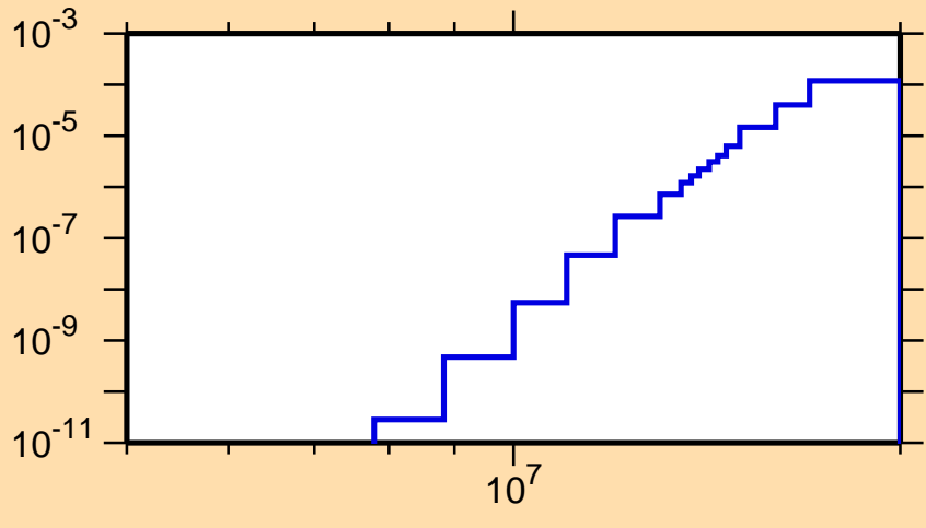
\sigma vs. E for ^{153}\text{Er}(n,\text{He3})
