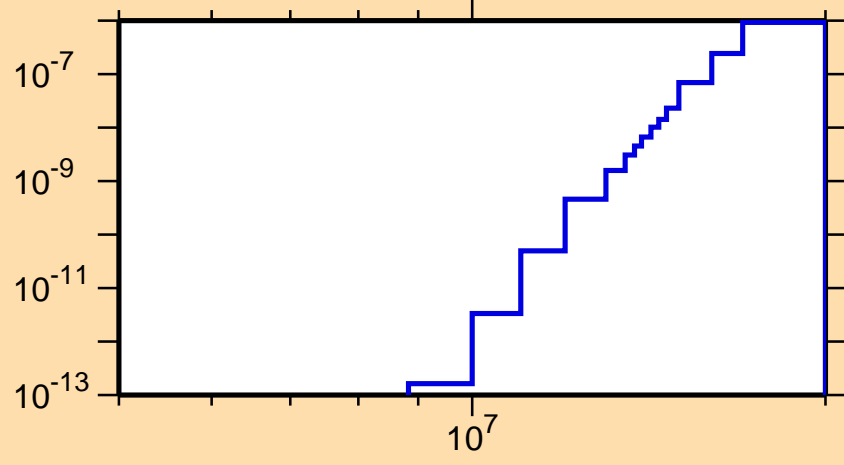
\sigma vs. E for ^{153}\text{Er}(\text{mt117})
