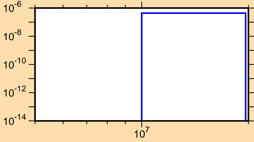
\sigma vs. E for ^{153}\text{Er}(n,\text{pd})
