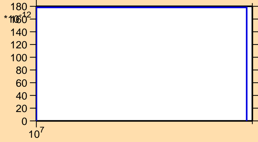
\sigma vs. E for ^{153}\text{Er} (mt 34)
