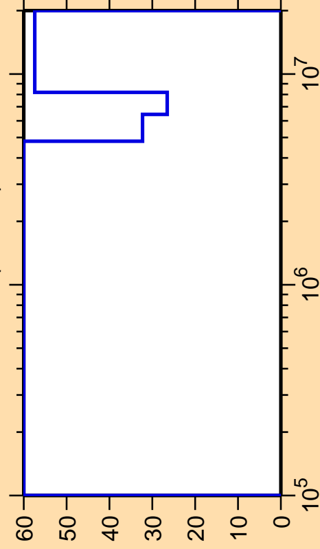
\Delta\sigma/\sigma vs. E for ^{153}\text{Er}(n,\text{inel.})
