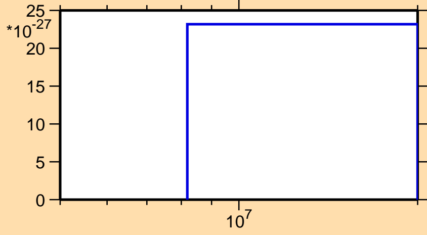
\sigma vs. E for ^{153}\text{Er} (mt 11)
