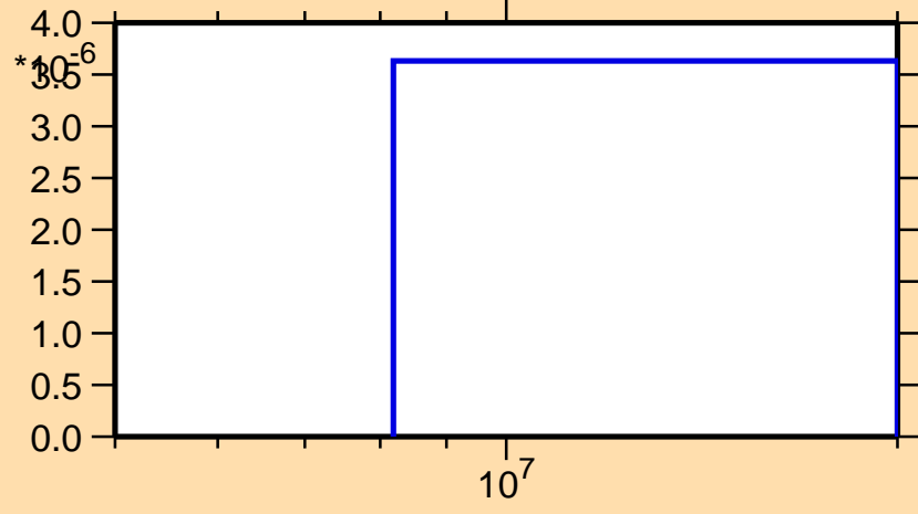
\sigma vs. E for ^{153}\text{Er} (mt 45)
