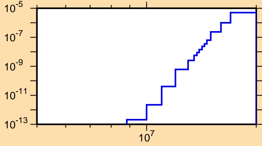
\sigma vs. E for ^{154}\text{Er}(\text{mt } 45)
