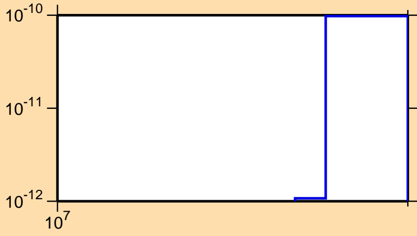
\sigma vs. E for ^{154}\text{Er} (mt 34)
