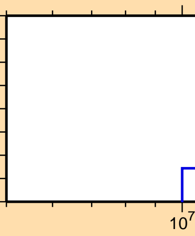
\sigma vs. E for ^{154}\text{Er}(\text{mt117})
