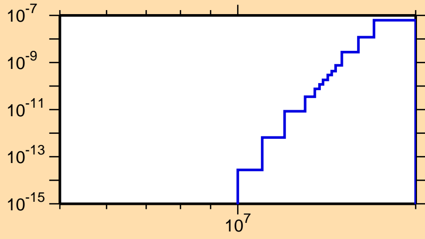
\sigma vs. E for ^{154}\text{Er}(\text{mt117})
