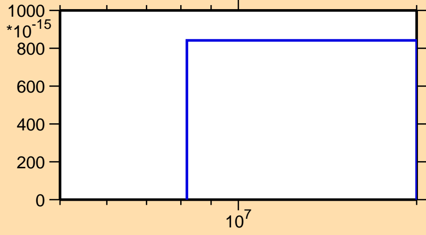
\sigma vs. E for ^{154}\text{Er}(\text{mt } 34)
