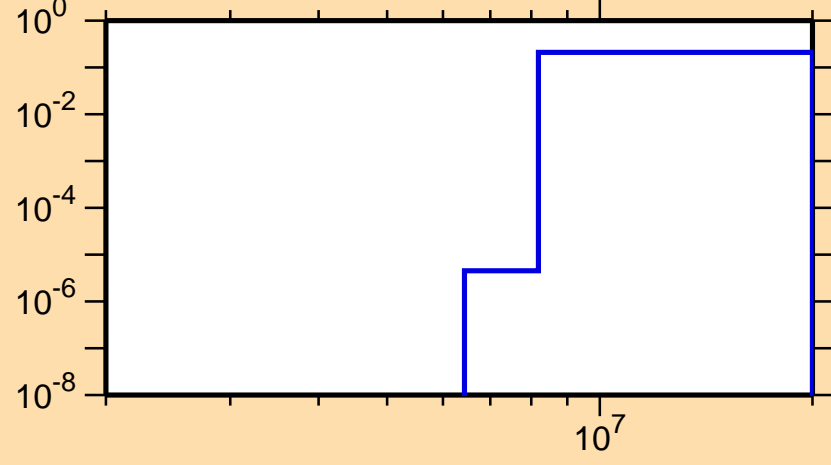
\sigma vs. E for ^{154}\text{Er}(n,np)
