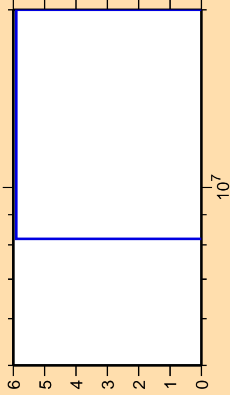
\Delta\sigma/\sigma vs. E for ^{154}\text{Er}(\text{mt } 34)
