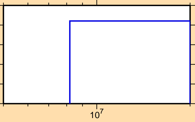
\sigma vs. E for ^{154}\text{Er}(\text{mt } 34)
