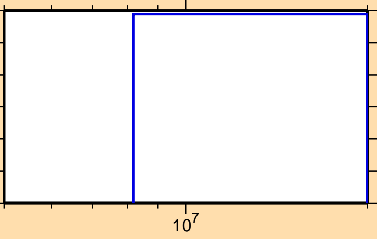
\sigma vs. E for ^{154}\text{Er} (mt 45)
