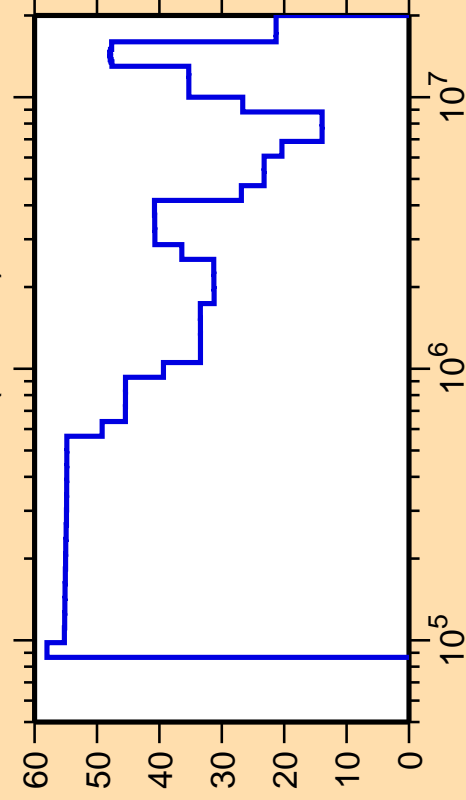
\Delta\sigma/\sigma vs. E for ^{155}\text{Er}(n,\text{inel.})
