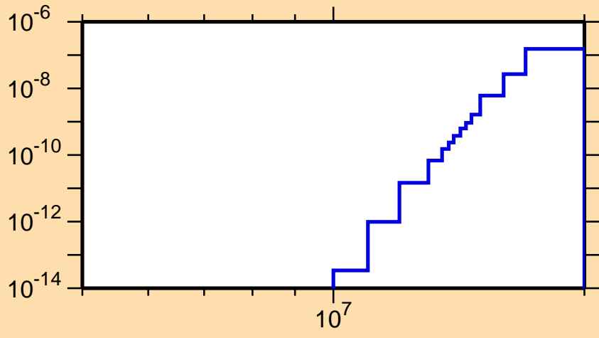
\sigma vs. E for ^{155}\text{Er}(\text{mt } 45)
