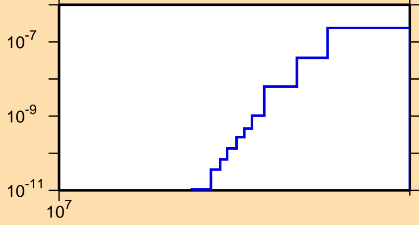
\sigma vs. E for ^{155}\text{Er}(n,\text{pd})
