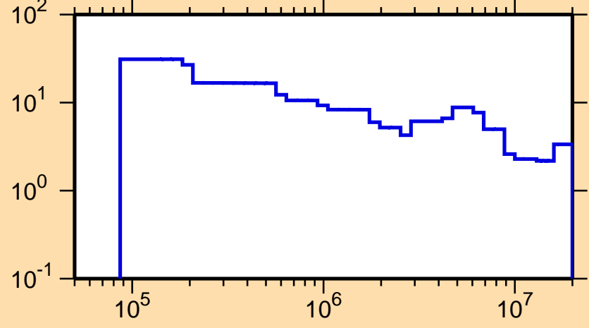
\Delta\sigma/\sigma vs. E for ^{155}\text{Er}(n,\text{tot.})
