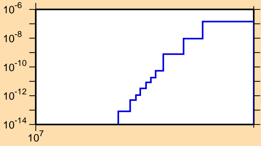
\sigma vs. E for ^{155}\text{Er}(n,\text{pt})
