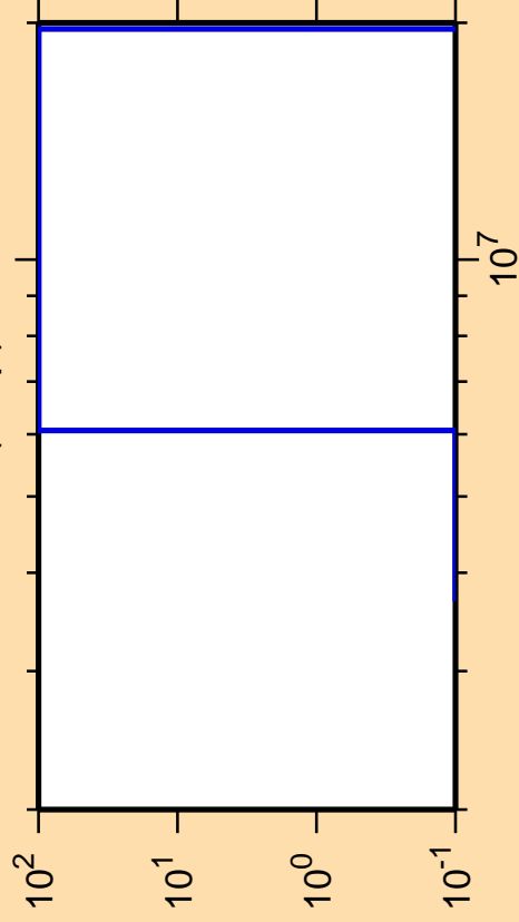
\Delta\sigma/\sigma vs. E for ^{155}\text{Er}(n,np)
