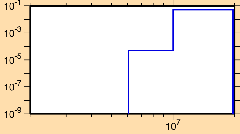
\sigma vs. E for ^{155}\text{Er}(n,np)
