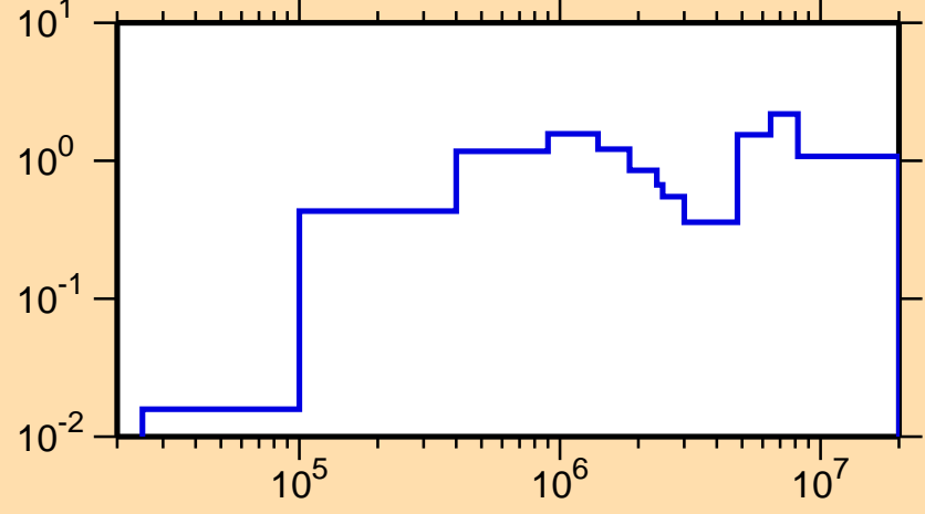
\sigma vs. E for ^{155}\text{Er}(n,\text{inel.})
