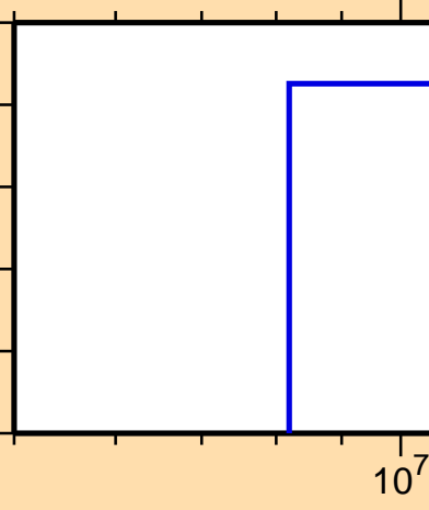
\sigma vs. E for ^{155}\text{Er}(n,\text{pd})
