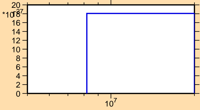
\sigma vs. E for ^{155}\text{Er}(\text{mt 11})
