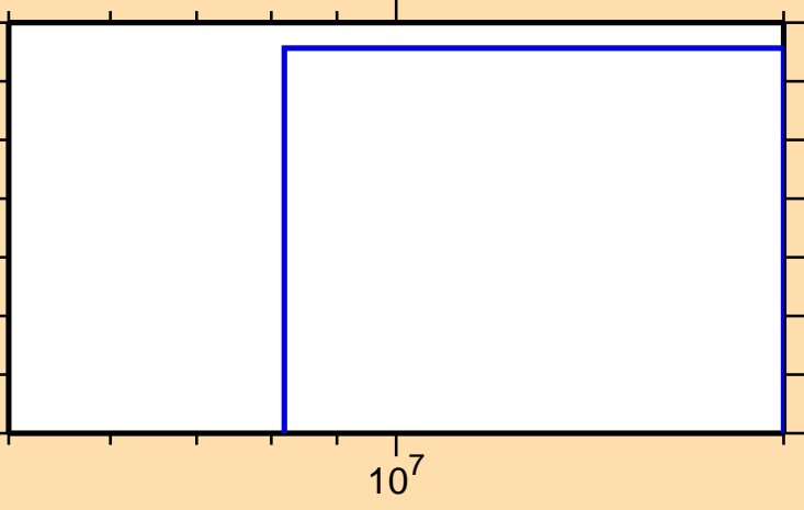
\sigma vs. E for ^{155}\text{Er}(\text{mt } 45)
