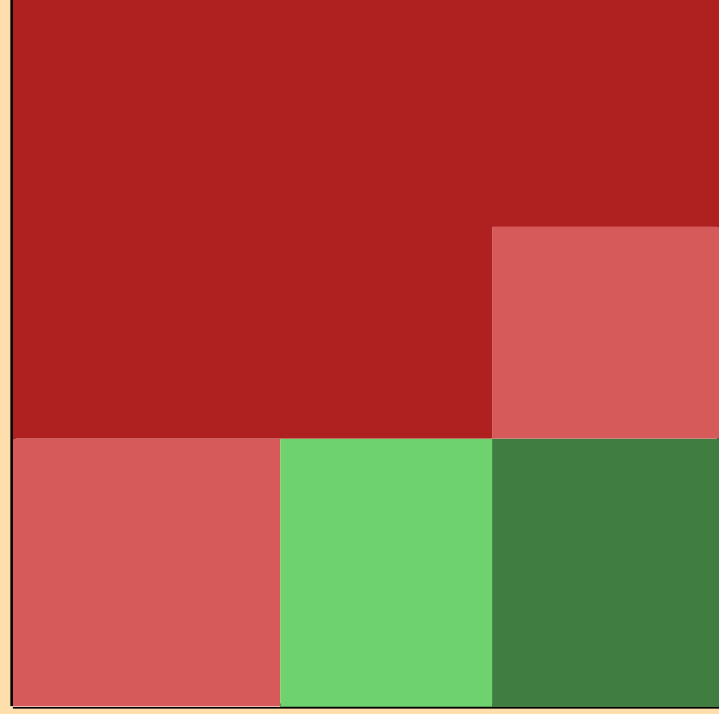
\Delta\sigma/\sigma vs. E for ^{156}\text{Er}(n,2n)
