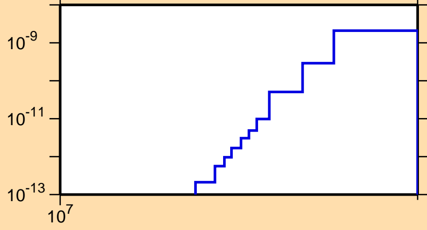
\sigma vs. E for ^{156}\text{Er}(\text{mt117})
