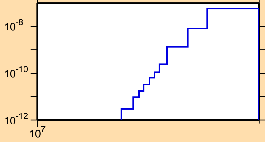
\sigma vs. E for ^{156}\text{Er}(\text{mt } 45)
