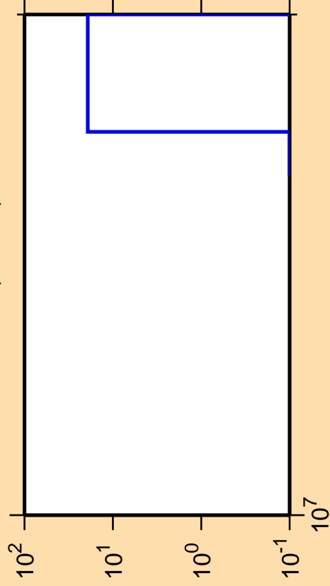
\Delta\sigma/\sigma vs. E for ^{156}\text{Er} (mt 34)
