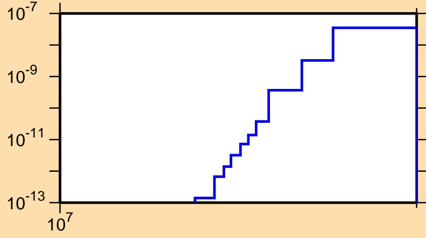
\sigma vs. E for ^{156}\text{Er}(n,pd)
