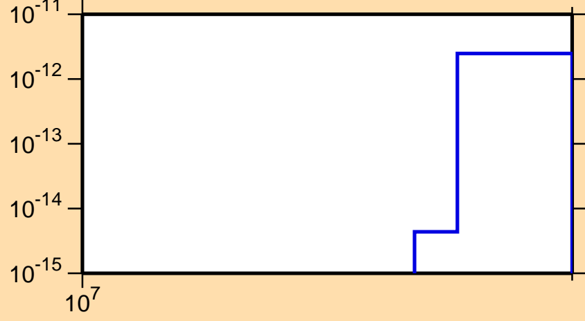
\sigma vs. E for ^{156}\text{Er} (mt 34)
