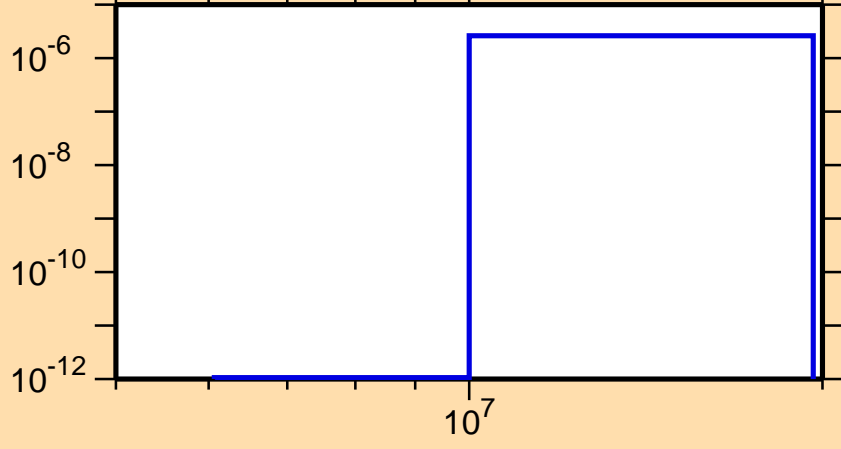
\sigma vs. E for ^{156}\text{Er}(n,2n\alpha)
