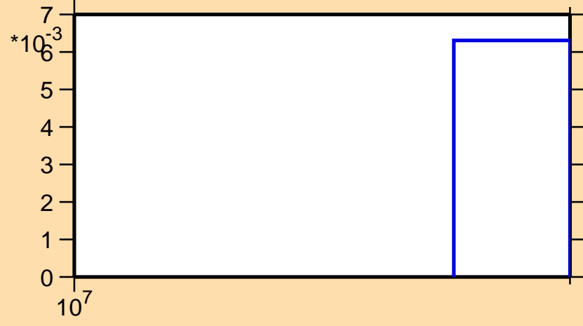
\sigma vs. E for ^{157}\text{Er}(n,3n)
