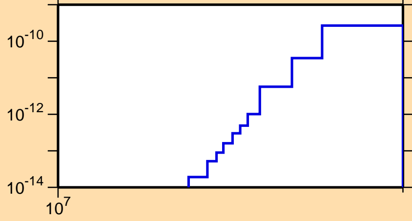
\sigma vs. E for ^{157}\text{Er}(\text{mt117})
