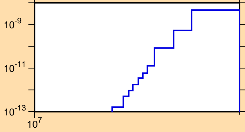
\sigma vs. E for ^{157}\text{Er}(\text{mt } 45)
