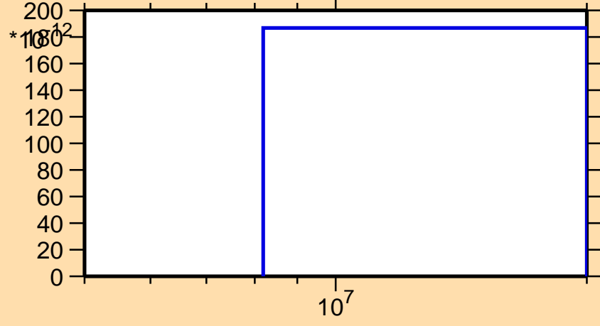
\sigma vs. E for ^{157}\text{Er}(n,pd)
