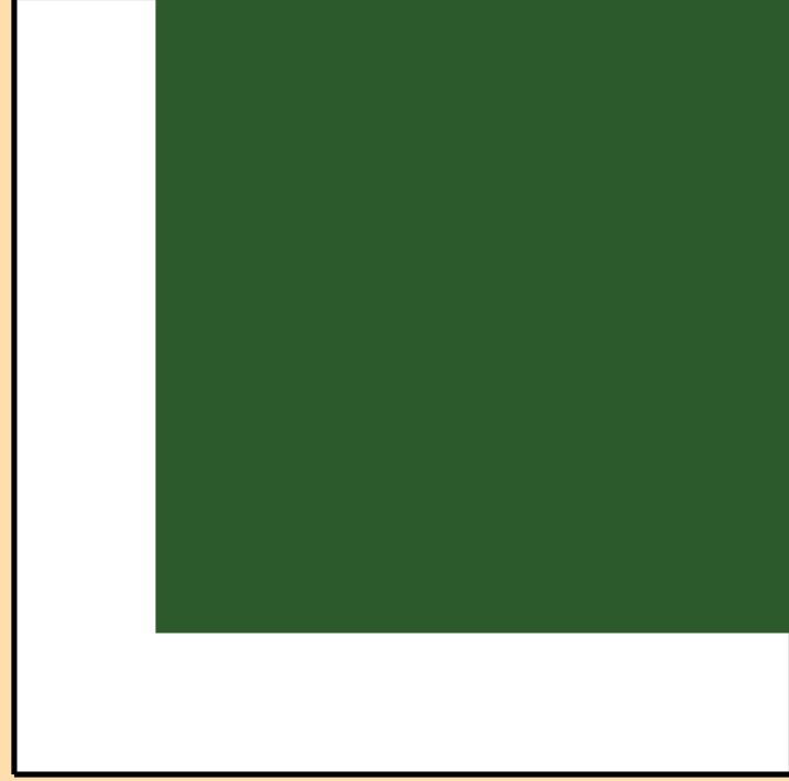
\sigma vs. E for ^{157}\text{Er}(n,2n)
