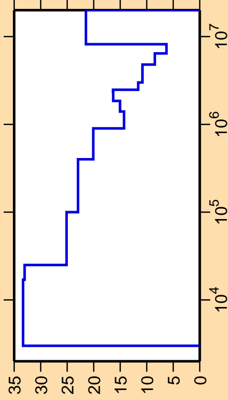
\Delta\sigma/\sigma vs. E for ^{157}\text{Er}(n,\text{inel.})
