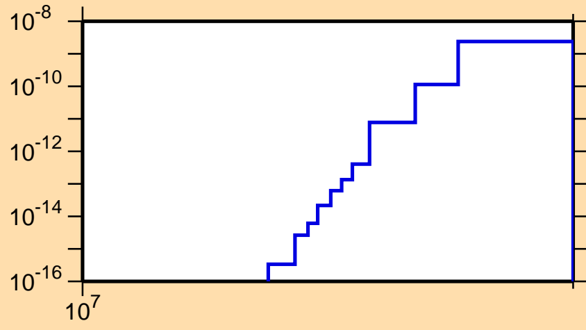
\sigma vs. E for ^{158}\text{Er}(n,pd)
