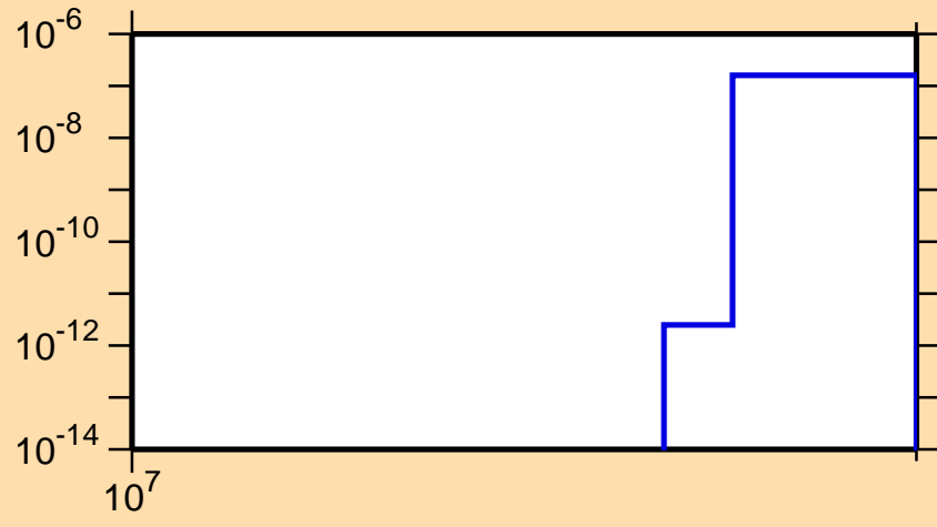
\sigma vs. E for ^{158}\text{Er}(n,2np)
