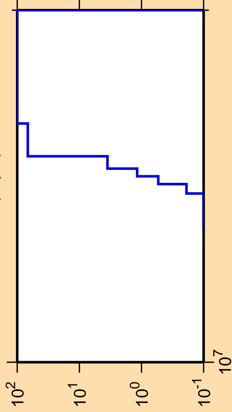
\Delta\sigma/\sigma vs. E for ^{158}\text{Er}(n,pd)
