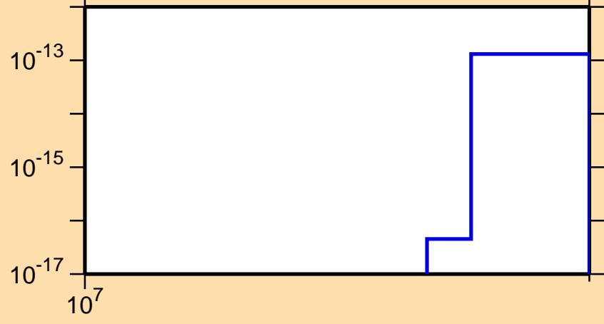
\sigma vs. E for ^{158}\text{Er}(\text{mt } 34)
