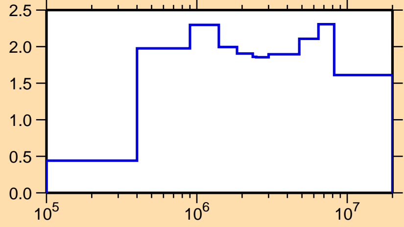
\sigma vs. E for ^{158}\text{Er}(n,\text{inel.})
