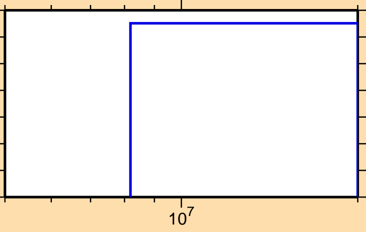
\sigma vs. E for ^{158}\text{Er}(n,2np)
