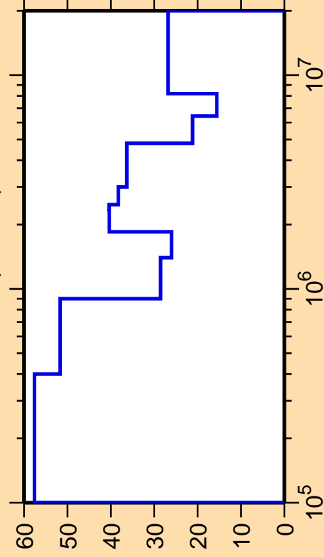
\Delta\sigma/\sigma vs. E for ^{158}\text{Er}(n,\text{inel.})
